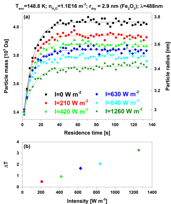
Figure 2. Panel a: Mean particle mass as a function of residence time in MICE for 6 different mean light intensities ( \lambda=488 nm, r_{dry}=2.9 nm ( \text{Fe}_2\text{O}_3 ), T_{env}=148.8 K, n_{\text{H}_2\text{O}}=1.1\text{E}16 m ^{-3} ). The solid curves represent fits of Eq. (2) to the data. Panel b: Particle temperature offsets \Delta T (Eq. (4)) as a function of the mean light intensities.
