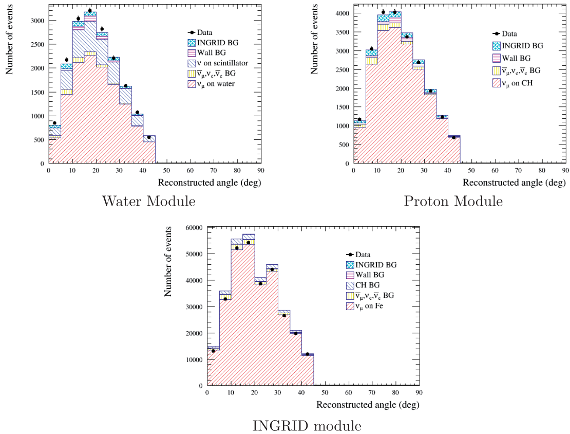
Fig. 10. Reconstructed angle of the longest track from a vertex after the event selection for the Water Module (upper left), Proton Module (upper right), and INGRID module (lower).
