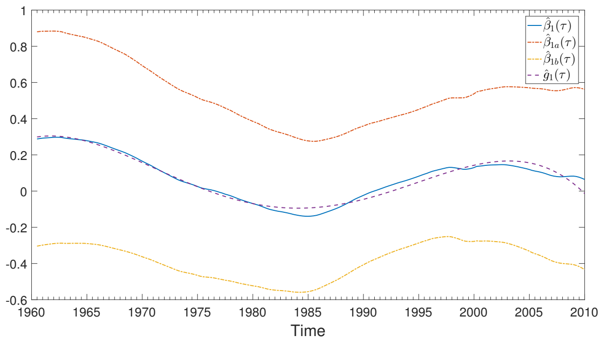
Figure 2: Nonparametric function estimate \hat{\beta}_1 with confidence intervals (\hat{\beta}_{1a}, \hat{\beta}_{1b}) together with the 4 th order parametric polynomial \hat{g}_1 estimate of \beta_1 .
