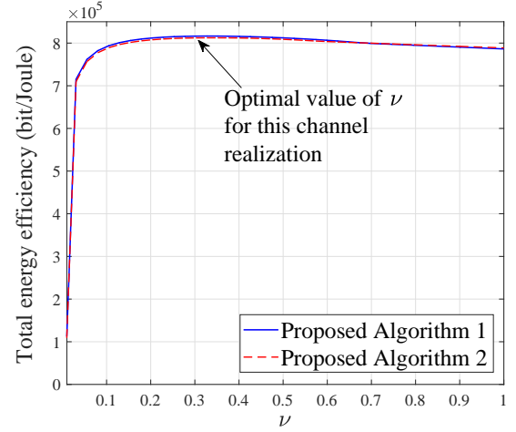
Figure 4. The total energy efficiency of proposed Algorithm 1 and proposed Algorithm 2 versus \nu for one channel realization with K = 20 , M = 100 , N = 1 , \alpha = 2 , \tau_p = 20 , and D = 1 km.
