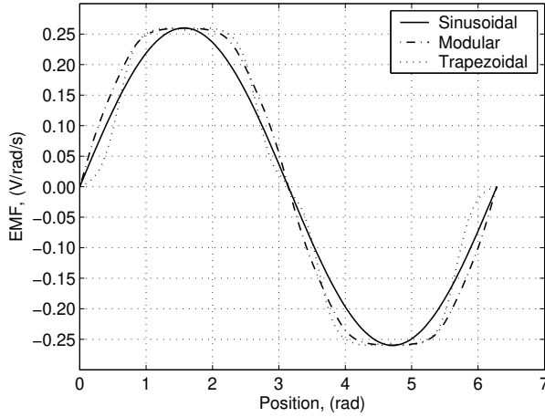
Fig. 11. Back-EMF Profiles
