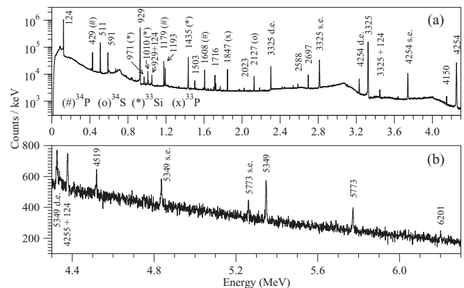
FIG. 2. \beta -gated \gamma -ray HPGe spectrum of the ^{34}\text{Al} decay recorded during the first 500 ms after the proton impact. The energy ranges shown are (a) 0–4.3 MeV and (b) 4.3–6.3 MeV. The most intense transitions in ^{34}\text{Si} are labeled together with the ones originating from longer-lived daughter nuclei. The latter are significantly suppressed because of the short 500 ms gating requirement and subsequent movement of the tape. The peaks corresponding to the \gamma rays from the long-lived daughters are indicated with symbols: (#) ^{34}\text{P} , (o) ^{34}\text{S} , (*) ^{33}\text{Si} , (x) ^{33}\text{P} . No contaminants could be identified.
