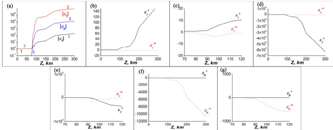
Figure 3. Part a) is the vertical dependencies of the components of modules of components of the permittivity in the frame associated with the geomagnetic field |\epsilon_j| , |\epsilon_2| , |\epsilon_h| , the curves 1, 2, 3 correspondingly. Parts b) – g) are the real and imaginary parts of the components \epsilon_j , \epsilon_3 , \epsilon_h , general and detailed views.
