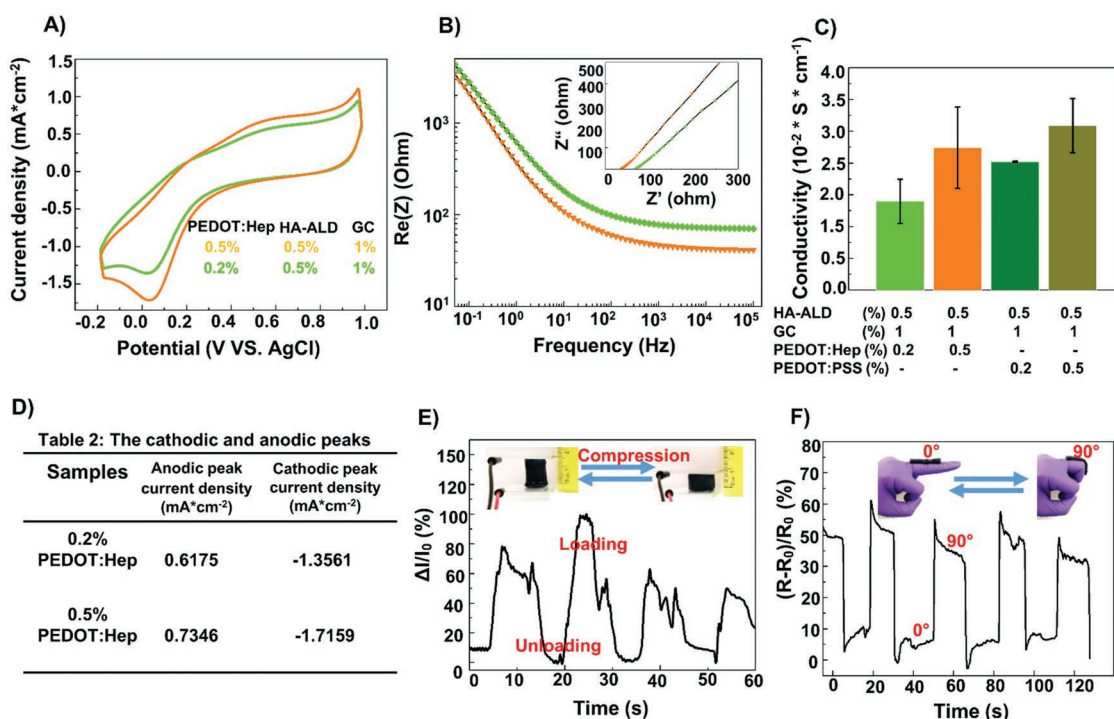
Figure 5. Electrochemical characteristics of the dual cross-linked electroconductive hydrogels. A) Cyclic voltammograms (current density vs the potential) of hydrogels with different concentrations of PEDOT:Hep, in PBS at a scan rate of 50 mV s -1 . B) Electrochemical impedance spectroscopy (Z vs frequency) of hydrogels with different concentrations of PEDOT:Hep (inset: Nyquist plot of the hydrogels). C) The conductivity of hydrogels (means, error bars, n = 3). D) The current density at the cathodic and anodic peak of the voltammograms of hydrogels with different concentrations of PEDOT:Hep. E) The relative current variation as function of time under a continuous cyclic tensile loading–unloading. Inset: Images of the compression and relaxation processes of the hydrogel, which undergoes a rapid recovery of its original shape to its a compressive deformation. F) Changes in the relative resistance during the bending of a finger at of angles at 0° and 90°.
