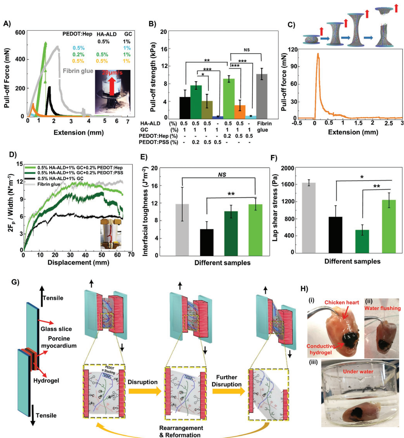
Figure 4. The adhesive property of electroconductive hydrogel. A) Adhesion pull-off testing of PEDOT:Hep hydrogels, where the adhesive strength is plotted against the extension. Inset: Detail of the experimental setup where the hydrogel adhered between two glasses that were pulled apart at a constant speed. B) The adhesive strength of the hydrogels. (Statistically significant differences are shown with asterisks * p < 0.05 , ** p < 0.01 , *** p < 0.001 , mean, error bar, n = 3 ). C) Scheme of the adhesion measurement, which shows the behavior of the hydrogel as the extension increases in correspondence with the adhesion force curve plotted against the extension (0.5% PEDOT:Hep 0.5% HA-ALD 1% GC). D) Double peeling force per band-shaped adhesive width obtained while peeling on porcine myocardium tissue band from the other glued by the different conductive hydrogels. (Inset: Photo of the double peeling test setup). E) The calculated interfacial toughness corresponding to (D) ( n = 4 ). Statistically significant differences are shown with asterisks * p < 0.05 , ** p < 0.01 , *** p < 0.001 , mean, error bars, n = 4 ). F) lap-shear strength of hydrogels and commercial fibrin glue sheared on flat porcine myocardium tissue ( n = 4 ). G) Image of the lab-shear experimental setup and adhesion mechanism of hybrid covalent/non-covalent dynamic network in conductive hydrogels. H) (i) Adhesion of the electroconductive hydrogel (0.5% PEDOT:Hep 0.5% HA-ALD 1% GC) on muscle tissue (chicken heart), (ii) the hydrogel remains adhered to the muscle tissue under flushing with water and (iii) under water.
