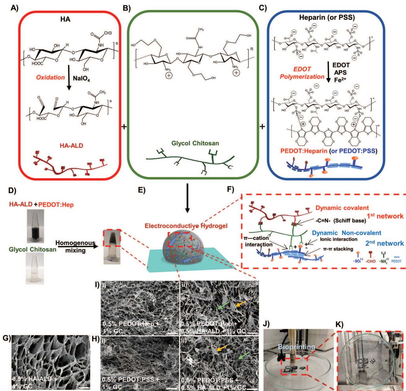
Figure 1. Characteristics of the dual cross-linked electroconductive PEDOT:Heparin/HA-ALD/GC hydrogels. A) Oxidation of HA by \text{NaIO}_4 , resulting in the formation of HA-ALD with the characteristic presence of aldehyde groups. B) Structure of glycol chitosan. C) PEDOT:Hep and PEDOT:PSS synthesis by polymerizing EDOT to form PEDOT particles using heparin or PSS as dopant. The chemical structures of PSS and PEDOT:PSS are not illustrated. D) Representative hydrogel formation by homogeneous mixing of HA-ALD + PEDOT:Hep with GC solutions in microtubes. E) Scheme of the 3D structure of the dual cross-linked hydrogel network. F) Scheme of the interactions involved in the formation of the double network. G–I) Scanning electron microscopy (SEM) images of hydrogel networks. The arrows in the dual cross-linked sample (I) indicate features, such as lamellar-like structures (yellow arrow) or fibers (green arrow). Scale bar: 10 \mu\text{m} . J) Bioprinting of a PEDOT:Hep + HA-ALD + GC hydrogel, which can adhere to the surface of a glass petri dish, and K) when holding the dish vertically.
