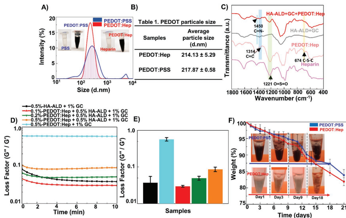
Figure 2. A) Particle size distribution of PEDOT:PSS and PEDOT:Hep solutions, determined by DLS. Inset: The solutions of PSS or heparin in MilliQ kept in microtubes and change from transparent to black after the polymerization of EDOT. B) The Z-average particle size of PEDOT:Hep and PEDOT:PSS. Mean \pm sd ( n = 3 ). C) Fourier transform infrared (FT-IR) spectra of Heparin, PEDOT:Heparin, HA-ALD+GC and HA-ALD+GC+PEDOT:Hep. D) PEDOT:Hep hydrogels (the loss factor plotted against the time). E) The loss factor at 10 min of gelation for hydrogels with PEDOT:Hep. The legend color is the same as Figure (D). F) Degradation assay of PEDOT:PSS or PEDOT:Heparin hydrogels. Inset: Images of PEDOT:PSS and PEDOT:Hep hydrogels during the degradation assay at 37 °C.
