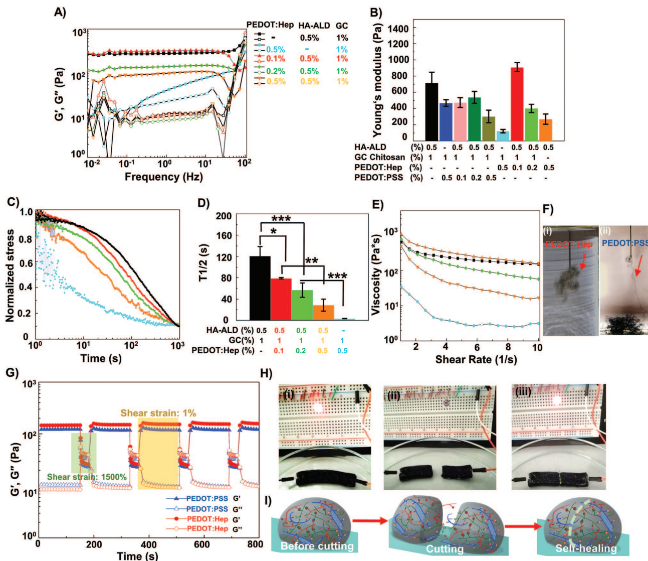
Figure 3. Rheological properties of the electroconductive hydrogels. A) Frequency sweep performed with a shear strain of 1% and the frequency increasing from 0.01 to 100 Hz. B) The Young's modulus of hydrogels at 10% shear strain (mean, error bar, n = 3 ). C) Stress relaxation curves of the hydrogels at a constant shear strain (1%). D) The stress relaxation half-times ( \tau_{1/2} ) of the hydrogels (Statistically significant differences are shown with asterisks *p < 0.05 , **p < 0.01 , ***p < 0.001 , mean, error bar, n = 3 ). E) Continuous flow experiments showing viscosity of the hydrogels plotted against the shear rate. F) The dual cross-linked hydrogels were syringe-injectable and thin filaments (indicated by the arrows) were extruded into PBS solution. G) Self-healing property of the hydrogels when the alternate step strain was switched from 1% to 1500%, indicated by the recovery of the elastic modulus. H) The self-healing of the hydrogel highlighted by an electric circuit with an LED. (i) The electroconductive hydrogel closed the circuit and the LED lit up. (ii) The hydrogel was cut into two pieces and the circuit opened. (iii) The hydrogel pieces were placed together and left to self-heal into one block (after 5 min) and the circuit was closed, as indicated by the LED. I) Scheme of the self-healing process of the electroconductive hydrogel.
