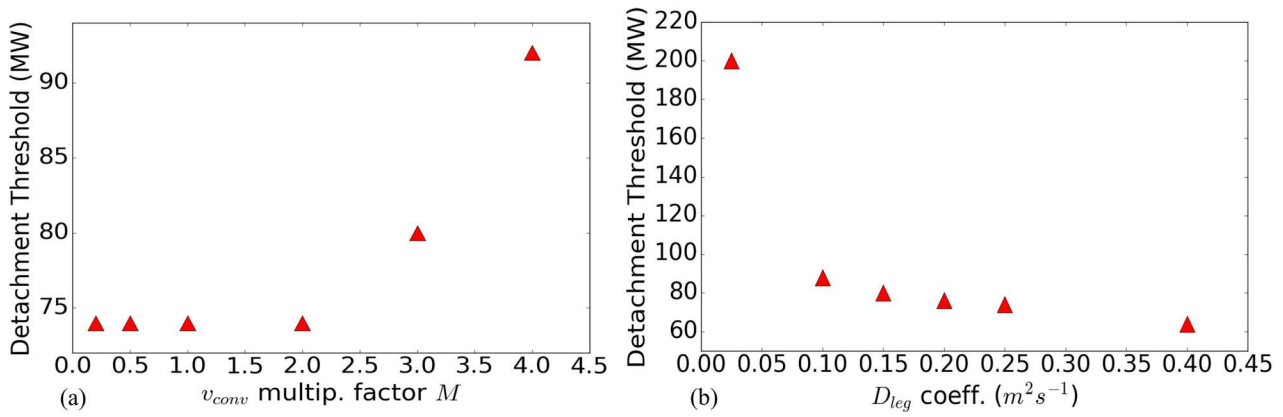
Figure 16. Variation in downswing power scan detachment threshold for variation in outer divertor leg values of (a) v_{conv} multiplier factor M and (b) diffusive transport coefficient D .
