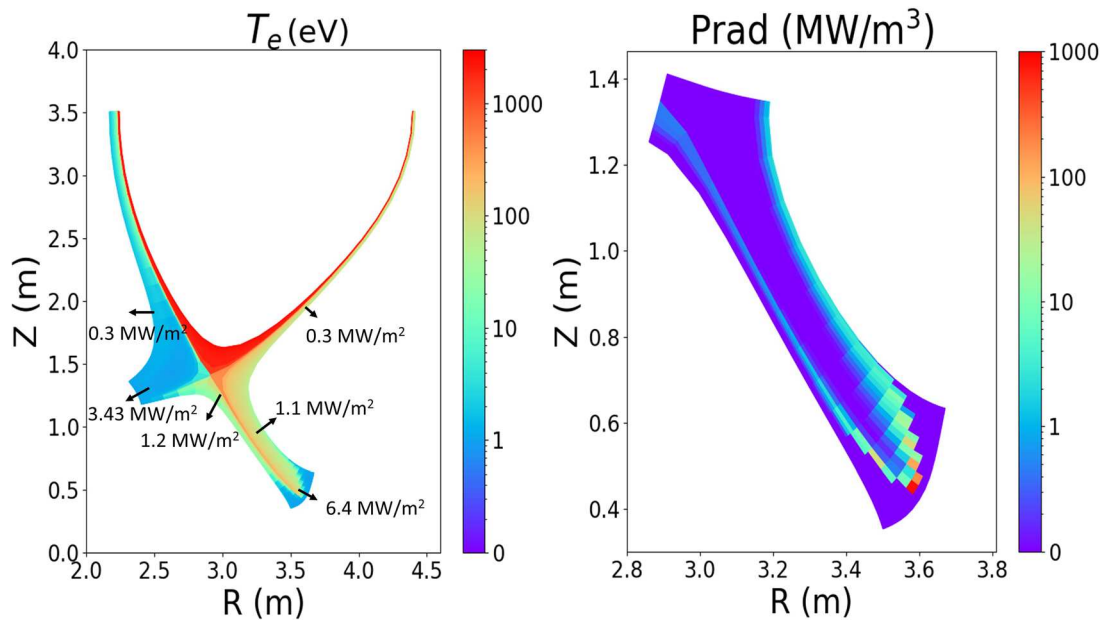
Figure 7. 2D plots for P_{SOL} = 105 MW, 0.5% Ne impurity detached SXD solution of (left) T_e with annotated peak power flux densities to the boundaries, for combined plasma and radiation power loadings, and (right) neon impurity radiation emissivity, with a peak value of 855 \text{ MW m}^{-3} .
