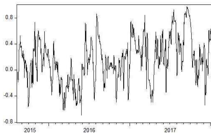
Fig. 3 Conditional Correlations
