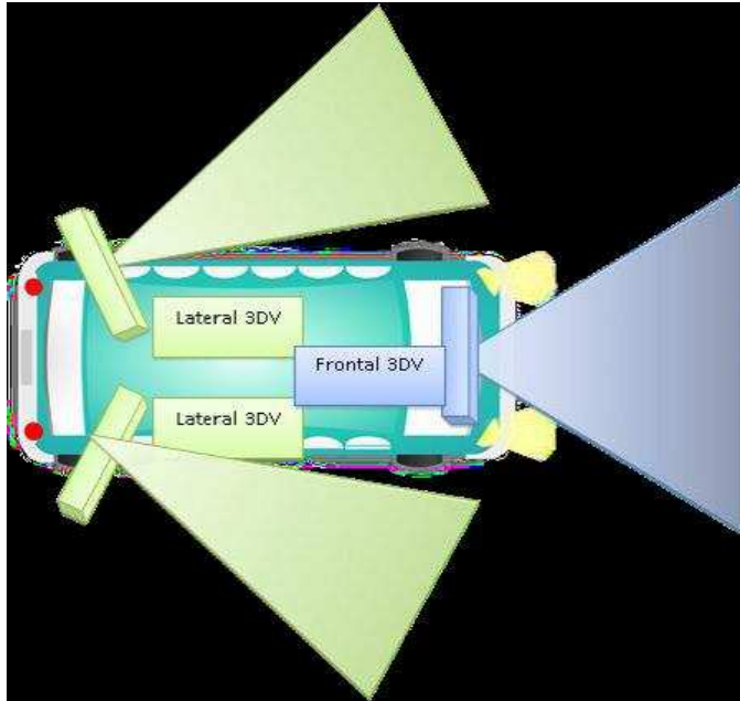
211 Figure 2: Aerial view of the positioning and area covered by the three 3DV cameras
