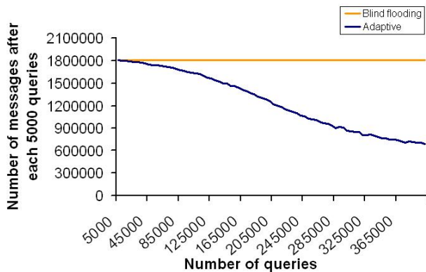
Figure 5. Messages passed in the network when using the flooding method and the adaptive method
