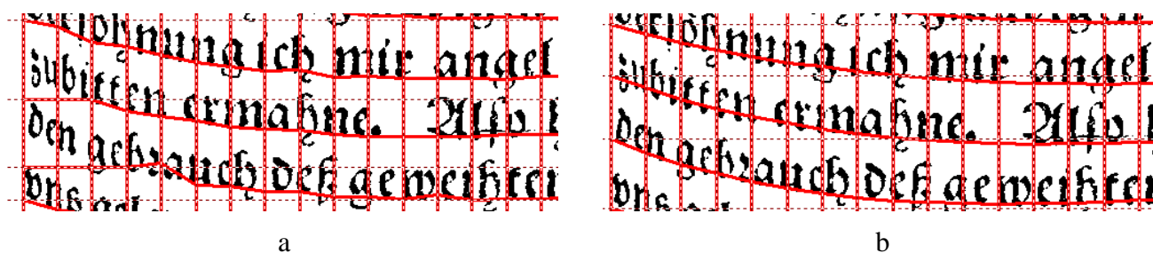
Fig. 8. Mesh adjustment by linear polynomial curve fitting. a) Mesh with global ambiguous points. b) Outlier correction by linear polynomial fitting
