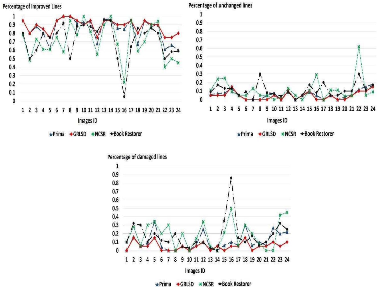
Fig. 16. Percentage of improved lines, unchanged lines and damaged lines of NCSR, Book Restorer TM and proposed method on SME. a) Percentage of improved lines. b) Percentage of unchanged lines. c) Percentage of damaged lines
