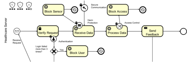
Fig. 30 Koh and Zhou business process model
