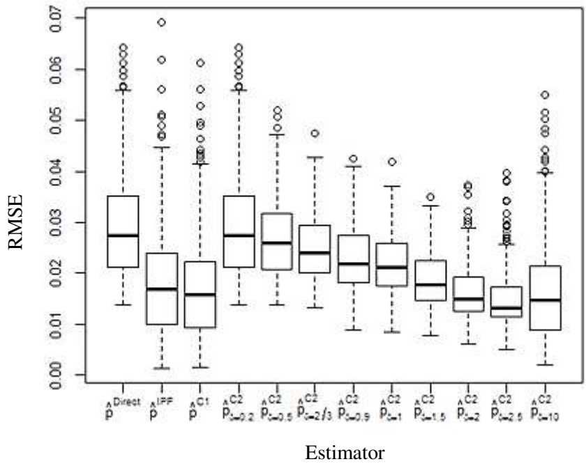
Figure 2 Box-plots of RMSE estimates.
