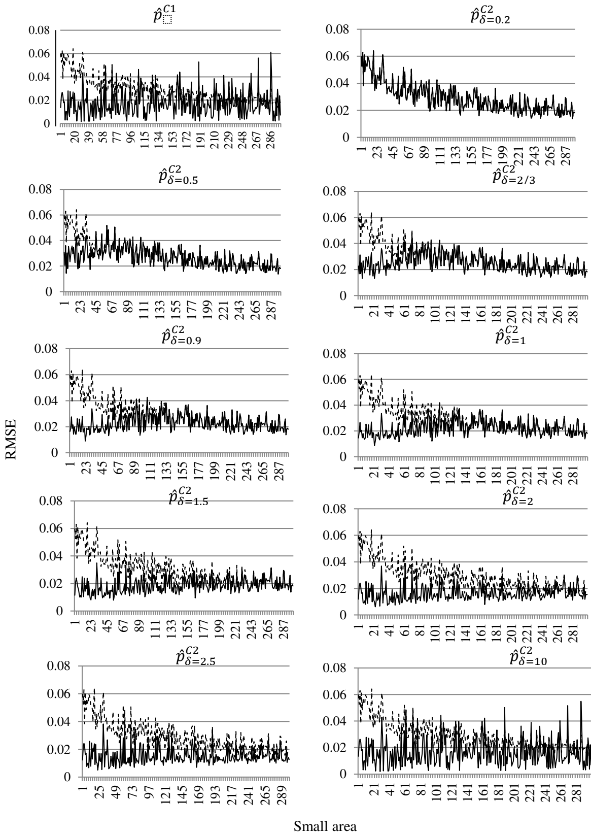
Figure A1 RMSE of composite estimates (—) and direct estimates (---).
