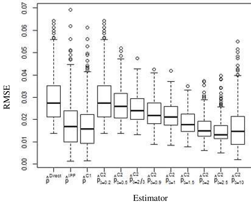
Figure 2 Box-plots of RMSE estimates.
