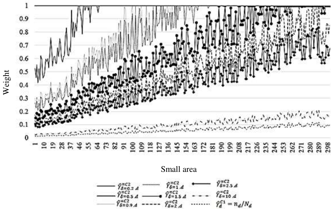
Figure 3 The behaviour of the weights within composite estimators across different small area survey sample sizes.
