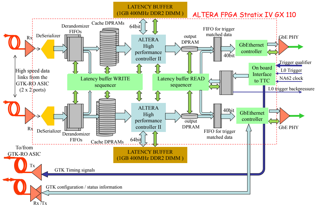
Figure 59. Block diagram of a GTK-RO motherboard. One GTK-RO serves one TDCpix ASIC.
