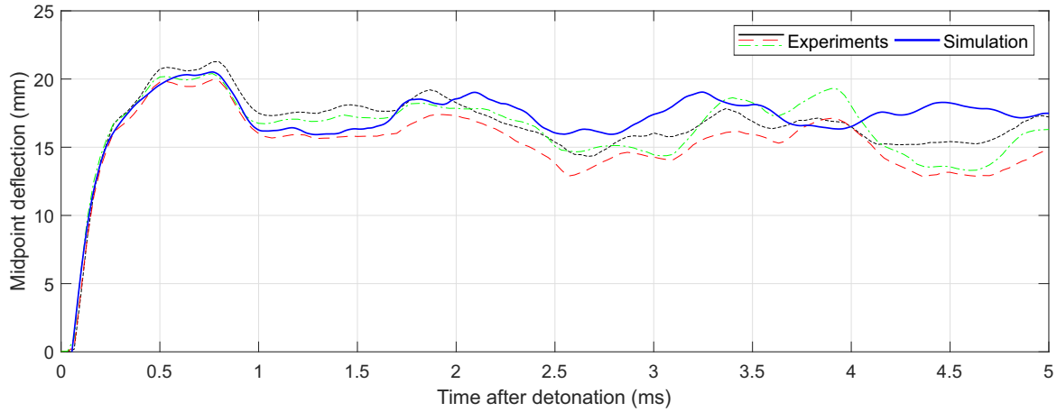
Figure 5: Validation of LS-DYNA against experimental results for 50 g PE4 sphere at 44.0 mm clear stand-off distance
