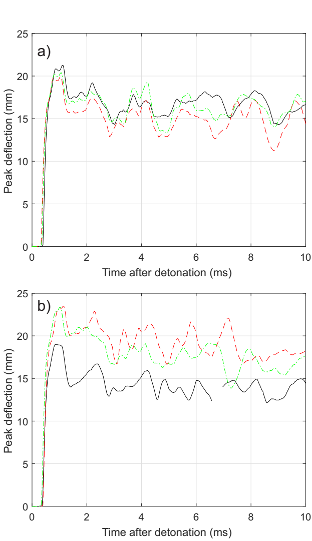
Figure 2: Peak deflection-time histories for tests with: a) spherical charges, and; b) cylindrical charges
