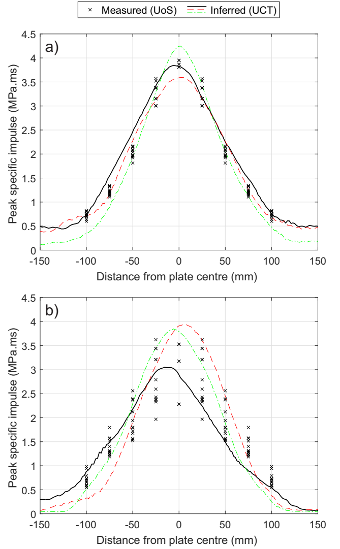
Figure 3: Measured (UoS) and inferred (UCT) specific impulses for: a) spherical, and; b) cylindrical tests, expressed at UoS scale
