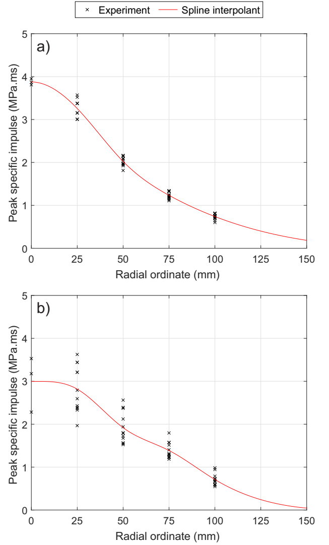
Figure 1: Compiled peak specific impulse at each bar location with fitted spline interpolant: a) Three tests with 100 g PE4 spheres at 55.4 mm clear stand-off; b) Three test with 78 g 3:1 PE4 cylinders at 168.0 mm clear stand-off
