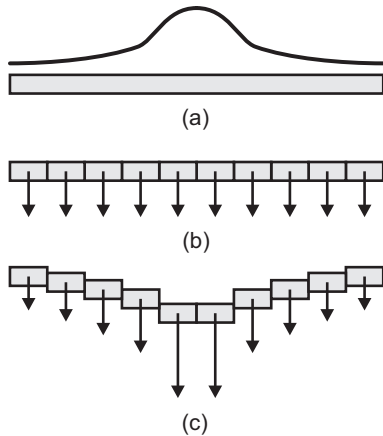
Figure 4: Initial distribution of specific impulse (a), and deformation modes associated with lower bound (b) and upper bound (c) kinetic energy
