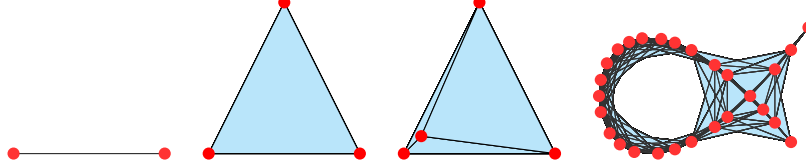
Figure 1: From left to right: Geometric realizations of a 1-simplex, 2-simplex, 3-simplex (the interior of the tetrahedron is included), and a general simplicial complex.
