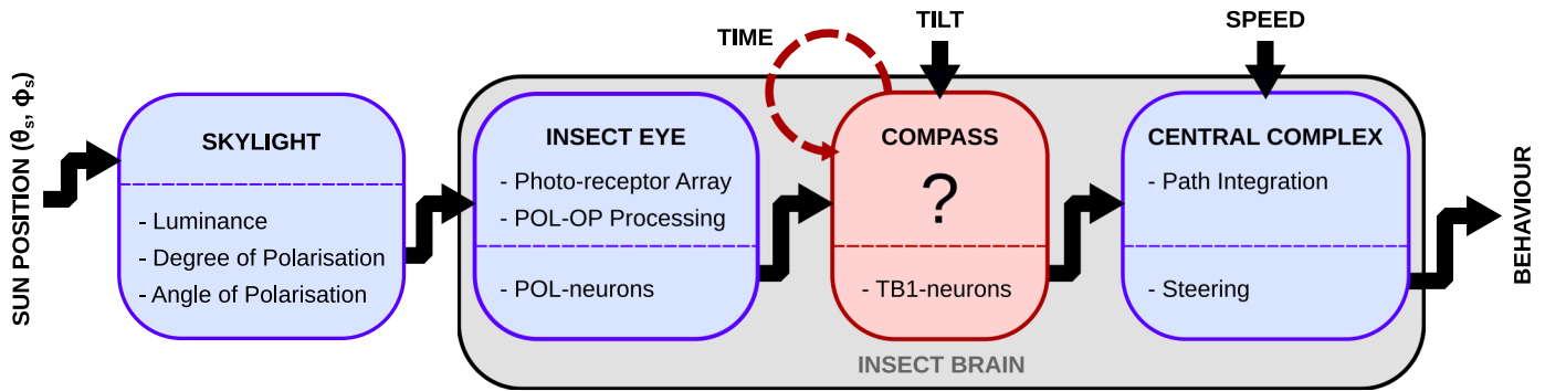
Fig 1. Overview of the modelling pipeline. Our simulation consists of four consecutive models (left to right). Given the position of the sun, a realistic skylight model [44] provides the predicted luminance, degree and angle of linear polarisation for every point in the sky-dome. This provides input to the eye model, based on biological data from insects [10, 38], which defines an array of polarisation sensitive photo-receptors facing different parts of the sky, and uses opponent processing to produce luminance-independent POL-neuron responses. The compass model provides a hypothesis for the unknown neural process that converts the POL-neuron response to a true compass signal in the TB1 neurons; this also utilises information about tilt of the sensor array, and allows for the movement of the sun with passing time. Finally, the compass neurons’ output is used along with speed as input to an anatomically grounded model of the central complex [35] which performs path integration and produces an output signal that can steer the insect back home. Blue boxes represent known systems in the pathway of the skylight; the red box represents a fuzzy/unknown system, which is the main focus of modelling in this paper.
