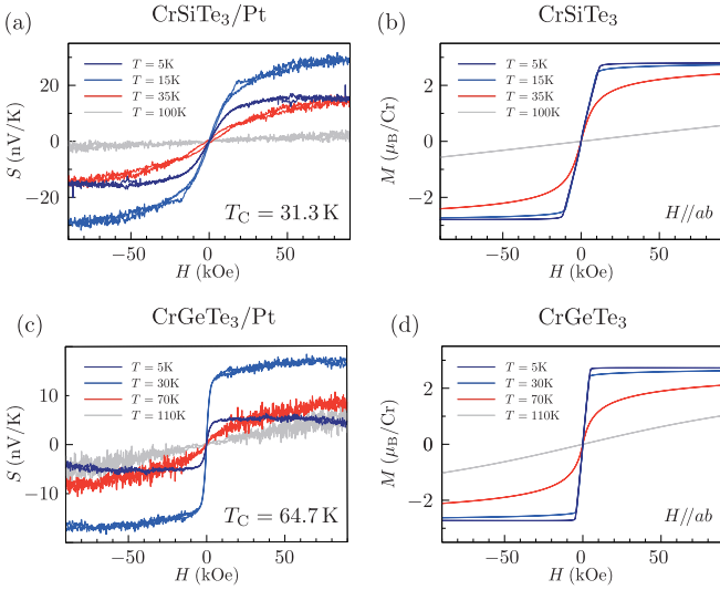
FIG. 3. H dependence of the normalized LSSE signal S in (a) \text{CrSiTe}_3/\text{Pt} and (c) \text{CrGeTe}_3/\text{Pt} and H dependence of M for (b) \text{CrSiTe}_3 and (d) \text{CrGeTe}_3 at several temperatures, where H was applied in the ab plane and swept between \pm 90 kOe.
