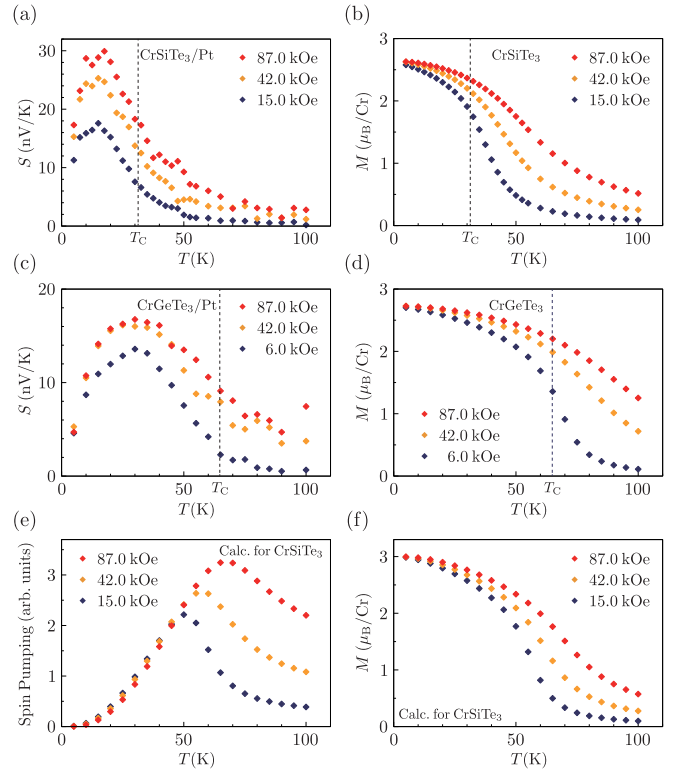
FIG. 4. T dependence of the normalized LSSE signal S (a) at 15.0, 42.0, and 87.0 kOe in \text{CrSiTe}_3/\text{Pt} and (c) at 6.0, 42.0, and 87.0 kOe in \text{CrGeTe}_3/\text{Pt} . T dependence of the magnetization M (b) at 15.0, 42.0, and 87.0 kOe in \text{CrSiTe}_3 and (d) at 6.0, 42.0, and 87.0 kOe in \text{CrGeTe}_3 . (e) Calculated spin pumping and (f) magnetization for \text{CrSiTe}_3 at 15.0, 42.0, and 87.0 kOe using the Hamiltonian in Ref. [22].
