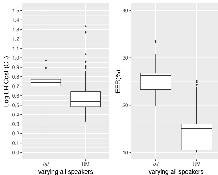
Figure 4: Boxplots of C_{lr} and EER of /a/ and UM by varying training, test and reference speakers in each replication.
