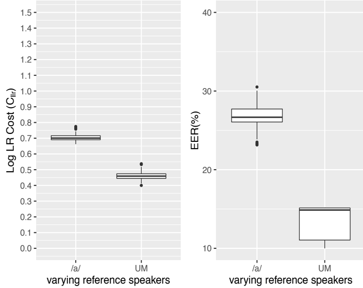
Figure 6: C_{lr} s and EERs for /a/ and UM varying reference speakers in each replication.
