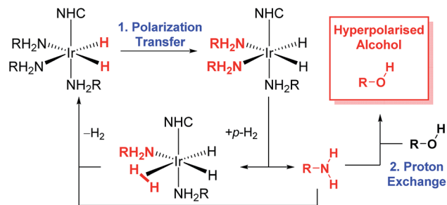
Scheme 1 The SABRE-Relay catalytic cycle for hyperpolarization for alcohols. Polarization is initially transferred from the p - H_2 derived hydride ligands to a carrier amine ( RNH_2 ) which subsequently transfer polarization to the alcohol via proton exchange. NHC is N-heterocyclic carbene.
