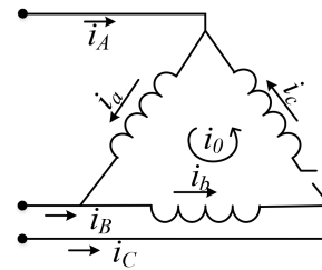
Fig. 6 Schematic of one phase OC scenario
