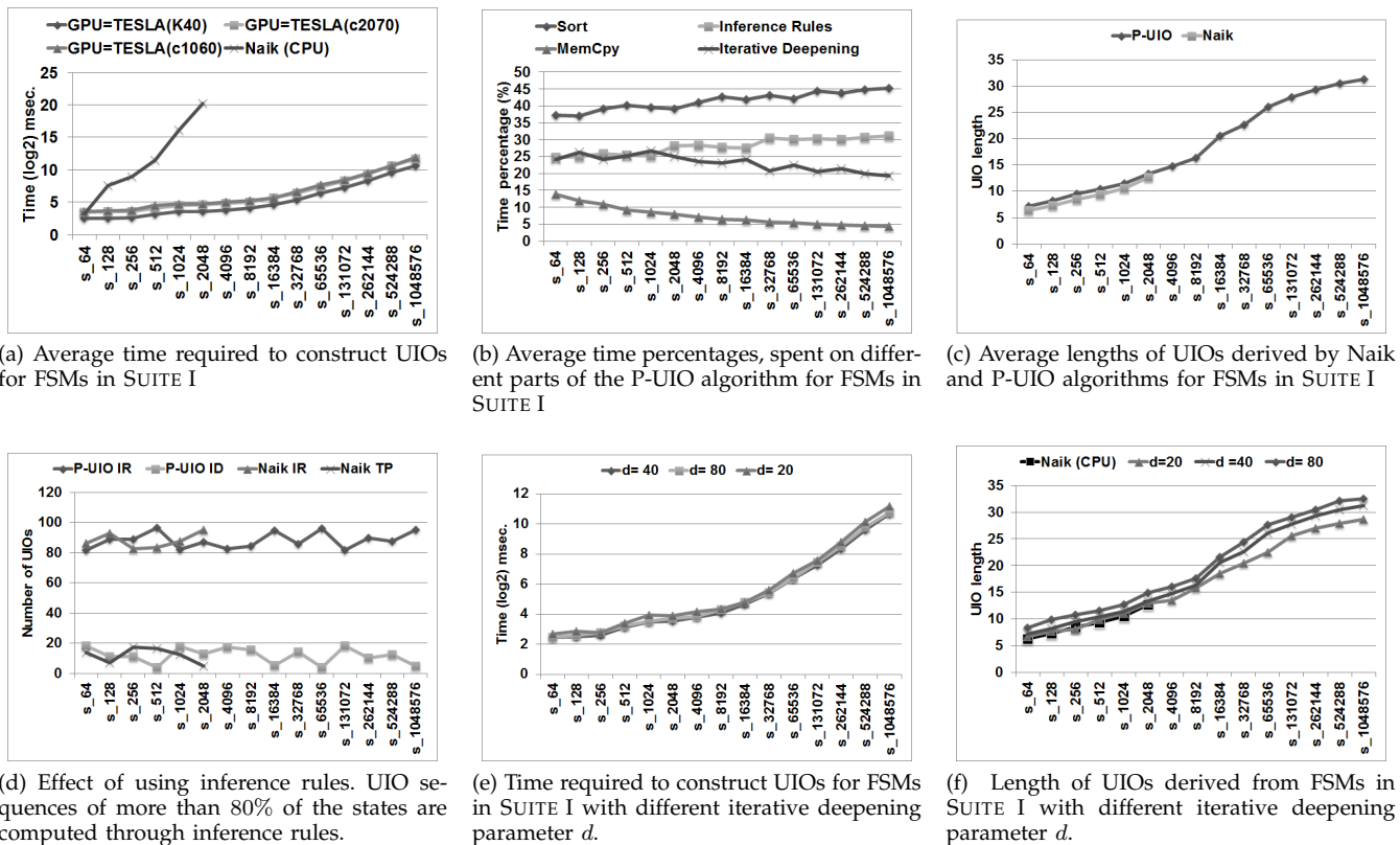
Figure 13: Results of experiments on test SUITE I.
