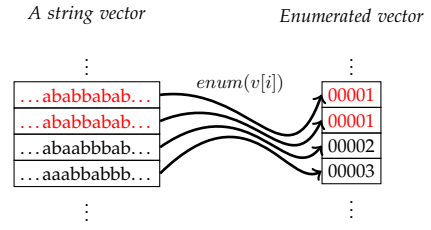
Figure 9: An illustration for enumeration. Each string is compacted to another string. Note that the enum function produces same values when given the same input string (red coloured texts).
