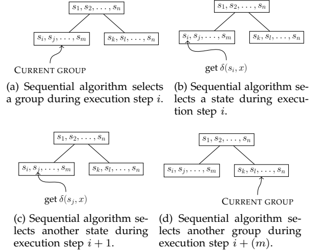
Figure 4: Steps of sequential algorithm overview. Note only current states are illustrated.
