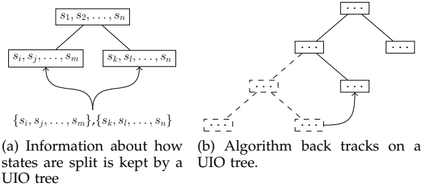
Figure 5: Use of tree structure while constructing a UIO tree. Note only current states are illustrated.
