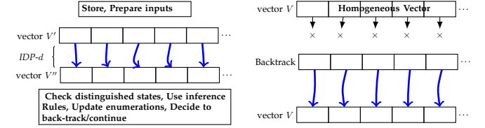
Figure 10: Overview of the steps taken in one iteration of P-UIO algorithm: the algorithm keeps evolving elements through the IDP. Before each iteration the algorithm stores the current data and chooses inputs to be applied. After each IDP, the algorithm checks for distinguished elements, applies inference rules, updates enumerations, and decides to continue or not. If the vector is homogeneous then it back-tracks.
