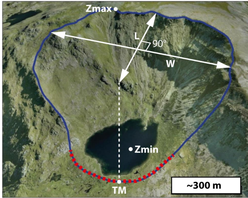
Fig. 1. Example cirque (Choire Dheirg, Scotland, 58.197°N, 4.974°W), mapped as a blue polygon. Cirque length (L) is the line within the cirque polygon that intersects the cirque threshold midpoint (TM—the threshold is marked as a dashed red line) and splits the polygon into two equal halves. Cirque width (W) is the line perpendicular to the length and intersecting the length line midpoint. Cirque depth (H), not shown in the figure, is the altitudinal difference between the minimum and maximum altitude within the cirque (i.e., Z_{max} - Z_{min} ). Spagnolo et al. (2017) provide further details of how these cirque metrics are calculated using their GIS tool. Background shows a getmapping TM aerial image, viewed obliquely in Google Earth TM.
