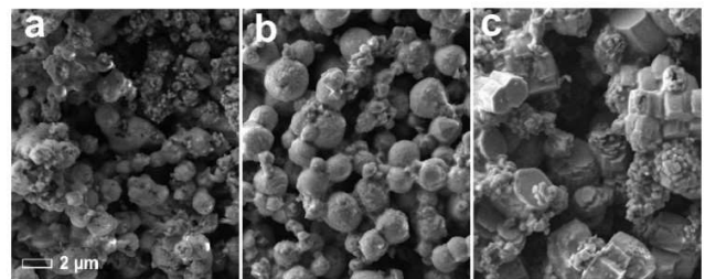
Figure 2. The morphology of as-prepared \text{Na}_2\text{S} (a), \text{Na}_2\text{S}_2 prepared at 110^{\circ}\text{C} (b) and \text{Na}_2\text{S}_2 prepared at 120^{\circ}\text{C} (c). Scale bar of 2\ \mu\text{m} is for all figures.
