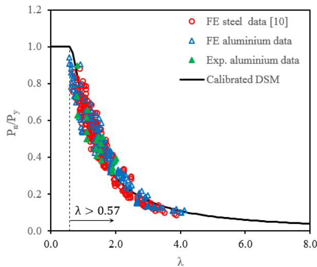
Figure 19: Comparison between the proposed DSM curve and FE/experimental data from aluminium and steel section database
