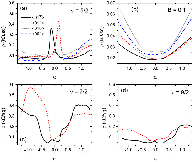
FIG. 3. 2DHS resistivity as a function of \alpha in the \langle 01\bar{1} \rangle (black, solid), \langle 011 \rangle (red, dashed), \langle 010 \rangle (grey, dotted), and \langle 001 \rangle (blue, dash-dot) directions, at (a) \nu = 5/2 ( B = 3.20 T), (b) B = 0 T, (c) \nu = 7/2 ( B = 2.22 T), and (d) \nu = 9/2 ( B = 1.73 T). The temperature is 50 mK and the 2DHS density is 1.91 \times 10^{11} cm ^{-2} . The data in (b) are taken with excitation current 5 nA.
