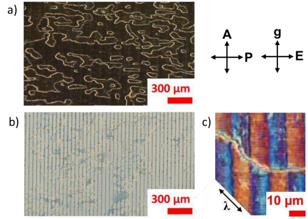
Figure 4. The texture of the SmC* in a) the OFF, and b) the ON state; c) the two opposite twists of the SmC* c -director in the presence of an electric field across an IDE and over a defect line.
