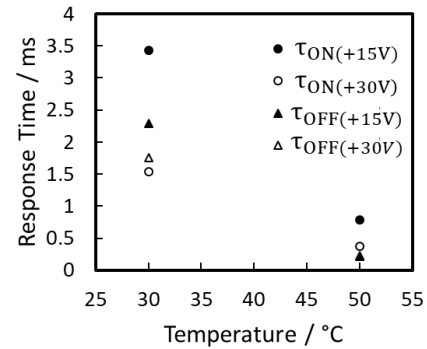
Figure 5. a) Response times for a VGA FLC device with d = 12 \mu\text{m} , P_{s(30^\circ\text{C})} = 7 nCcm -2 , on the application of 15V and 30V driving pulses, at 30°C and 50°C, where the error bars are the size of the data points. Sub-millisecond response times are obtained for the device at 50°C.
