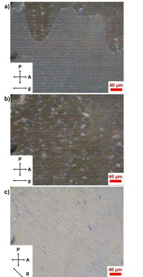
Figure 3. a) A carpet-like texture of the FLC held at 55^\circ\text{C} , showing the changes in texture on either side of a moving disclination line as new smectic layers form resulting in a more uniform texture. The direction of flow is from top to bottom. A similar effect is seen when the device is susceptible to a shock. b) With time, the undulations completely disappear, until the device is further cooled or shocked. The texture is not black due to slightly misaligned gratings, and a high light intensity to clearly show the undulating texture. c) a 45^\circ rotation of the device to show \mathbf{c} -director alignment is maintained.
