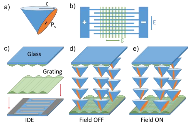
Figure 1. Schematic diagram of the VGA-FLC device geometry. a) Representation of the c -director, c , and the spontaneous polarisation, P_s , of the FLC; b) Orientation of the gratings with respect to the in-plane electrodes; c) 3D schematic of the gratings with respect to the IDE; d) Device in the OFF/dark state, with no applied electric field, where the c -director is homogeneously aligned through the cell; e) Device with an electric field applied to rotate the c -director 90° through the cell. On removal of this field, the device relaxes back to the homogeneous c -director alignment shown in d). Note that opposite twist will occur on opposite sides of an IDE.
