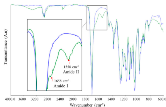
Figure 3. ATR-FTIR analysis of unconjugated (blue) and conjugated (green) fibrous scaffolds.
