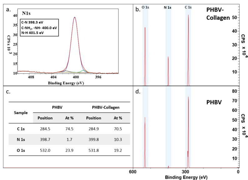
Figure 4. XPS analysis of PHBV and PHBV-Collagen fibre membranes: (a) a high-resolution view of the N 1s peak observed upon conjugation of collagen; (b) spectra for PHBV-Collagen; (c) table of peak binding energies and the percentage of elements present; and (d) spectra for PHBV.
