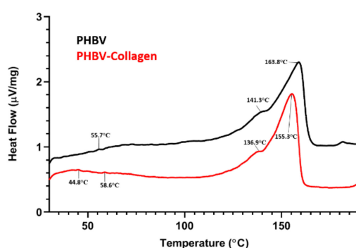
Figure 5. DSC thermograms of PHBV and PHBV-Collagen membranes.
