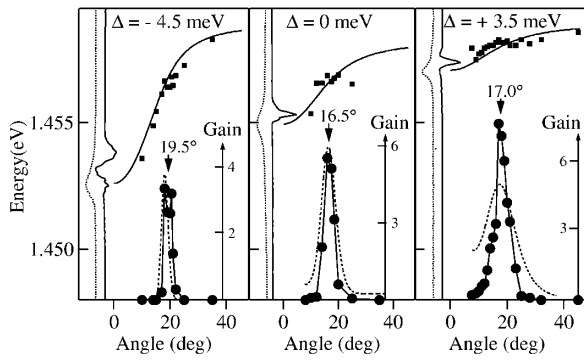
FIG. 3. Parametric gain ( \bullet ) vs angle for detunings \Delta = -4.5, 0, +3.5 meV. The energy of the pump pulse ( \blacksquare ) is tuned to achieve maximum gain. Fitted dispersion relations (lines) match the reflected probe spectra shown solid (dashed) on the left side for pump on (off). The gain peaks are at 19.5 \pm 1.5^\circ , 16.5 \pm 2^\circ , and 17 \pm 2.5^\circ , respectively, compared to the predicted curves shown dashed, which are at 18.0^\circ , 16.3^\circ , and 17.2^\circ . Pump (probe) powers are 20 \text{ W/cm}^2 ( 0.4 \text{ W/cm}^2 ).
