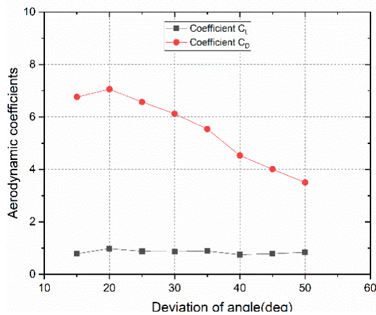
Fig.17 Influence of wind yaw angle on aerodynamic coefficients
