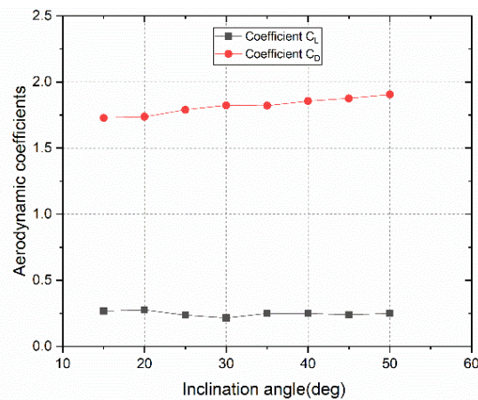
Fig.11 Influence of inclination angle on aerodynamic coefficients
