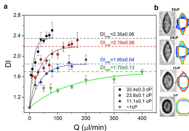
FIGURE 3 (a) Deformation index versus Q for HL60 cells in four different media with viscosity changing between 1 and 33 cP. DI \pm standard error was averaged from multiple cell events combined from N = 3 repeats; each data point includes 30 > n > 500 cell events. The data is fitted with an exponential. (b) Images of a cell deformation for each flow condition where DI \approx DI_{\text{max}} are shown. They are accompanied by superimposed color contour plots that show how the deformation changes as a function of time. To see this figure in color, go online.
