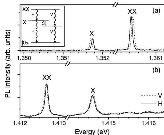
FIG. 1. Photoluminescence spectra from two single quantum dots (a) from an unannealed sample and (b) from a sample annealed for 5 min at 750 °C. Solid and dotted lines represent horizontally ( H ) and vertically ( V ) polarized detection for (a) and (b), respectively. Two groups of lines are observed corresponding to emission from exciton ( X ) and biexciton ( XX ) states as labeled. The inset to the figure shows a simple energy level diagram illustrating optical decay from the XX state; the exciton level splitting S is labeled.
