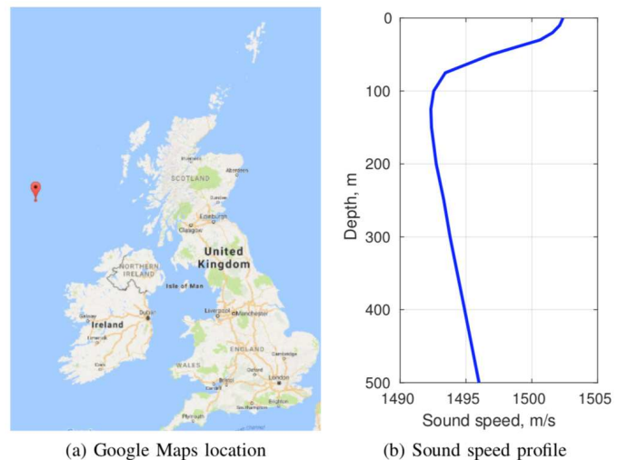
FIGURE 5. Example of an SSP in the North Atlantic Ocean [7]
