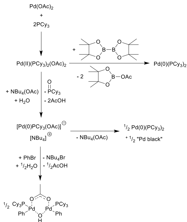
Scheme 6. Reduction routes for palladium acetate in non-polar solvents where bis(pinacolato)diboron or tricyclohexylphosphine are oxidised.
