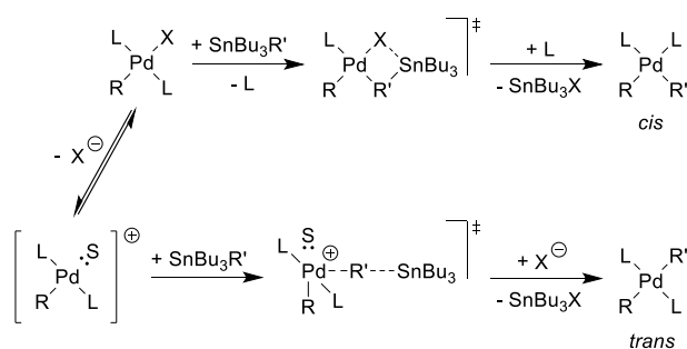
Scheme 22. The open (lower route) and closed (upper route) mechanisms of transmetalation in a Stille reaction.
