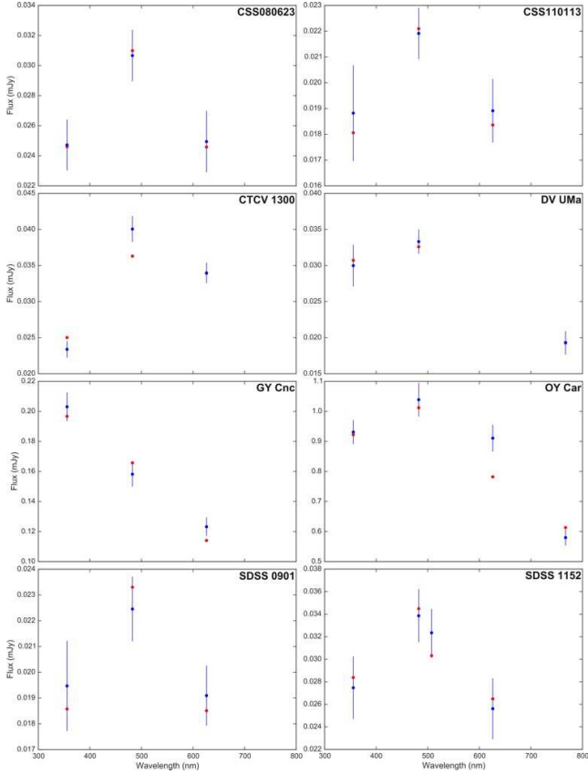
Figure 2. White dwarf fluxes for 13 CVs, showing the white dwarf fluxes from the eclipse model fits (blue) and white dwarf atmosphere predictions (red), at wavelengths corresponding to u' (355.7 nm), g' (482.5 nm), KG5 (507.5 nm), r' (626.1 nm) and i' (767.2 nm) filters. The name of each system is displayed in the top-right corner of each plot.
