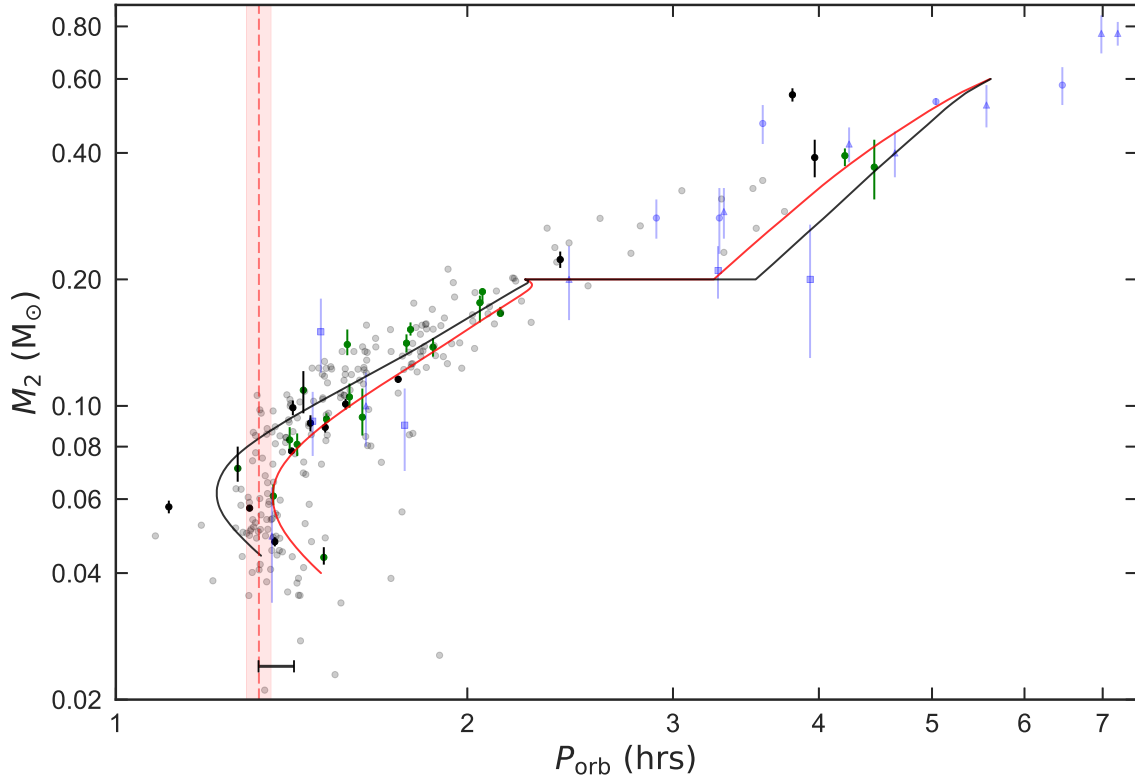
Figure 10. Measured CV donor masses ( M_2 ) as a function of orbital period ( P_{\text{orb}} ). The data point colour/shape scheme is the same as in Figure 8. The red and black lines represent the best-fit ( f_{\text{GR}} = 2.47 \pm 0.22 , f_{\text{MB}} = 0.66 \pm 0.05 ) and ‘standard’ ( f_{\text{GR}} = f_{\text{MB}} = 1 ) evolutionary tracks from Knigge et al. (2011), respectively. The vertical dashed red line and shaded region is an estimate of the true P_{\text{min}} based on fitting a Gaussian distribution to the orbital periods in the range 76–82 mins.
