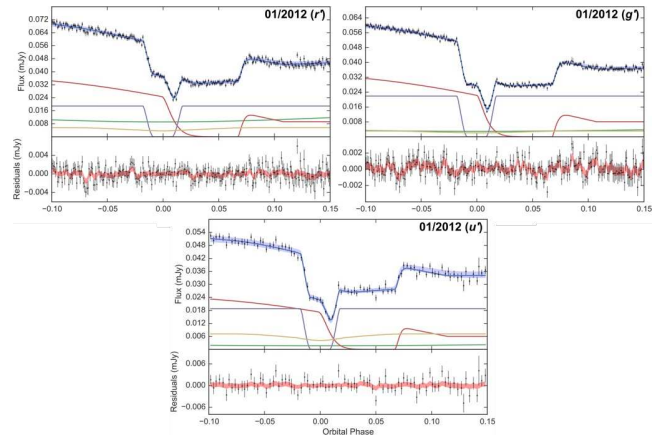
Figure A3. Simultaneous eclipse model fit to three average CSS110113 eclipse light curves. See Section 4.1 for full details of what is plotted. Displayed in the top-right corner of each average eclipse plot is the date and wavelength band each of the constituent eclipses were observed in.
