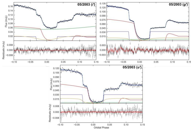
Figure A4. Simultaneous eclipse model fit to three average DV UMa eclipse light curves. See Section 4.1 for full details of what is plotted. Displayed in the top-right corner of each average eclipse plot is the date and wavelength band each of the constituent eclipses were observed in.
