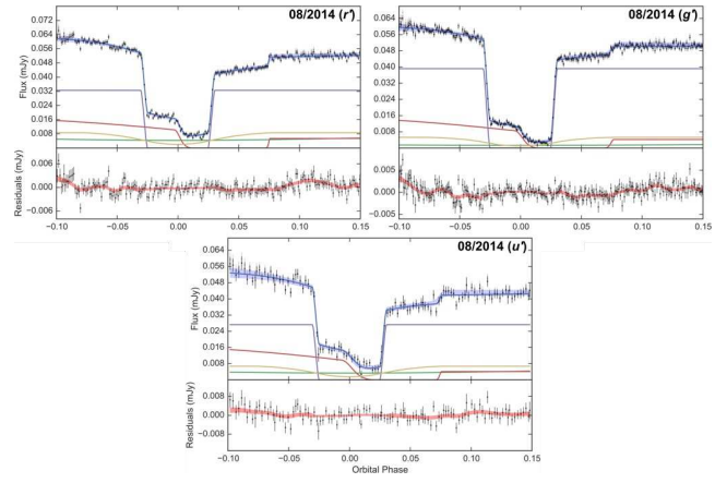
Figure A11. Simultaneous eclipse model fit to three average SSS100615 eclipse light curves. See Section 4.1 for full details of what is plotted. Displayed in the top-right corner of each average eclipse plot is the date and wavelength band each of the constituent eclipses were observed in.
