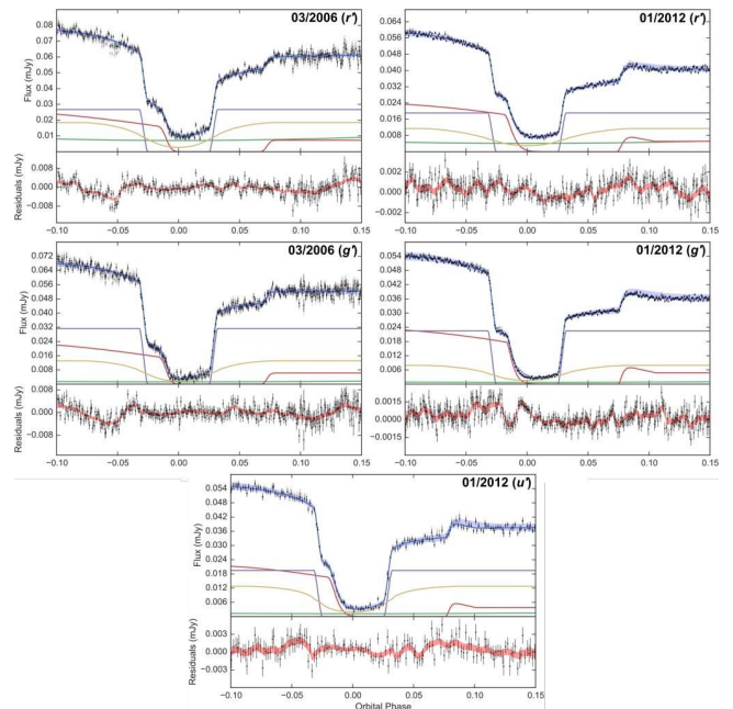
Figure A7. Simultaneous eclipse model fit to five average SDSS 0901 eclipse light curves. See Section 4.1 for full details of what is plotted. Displayed in the top-right corner of each average eclipse plot is the date and wavelength band each of the constituent eclipses were observed in.
