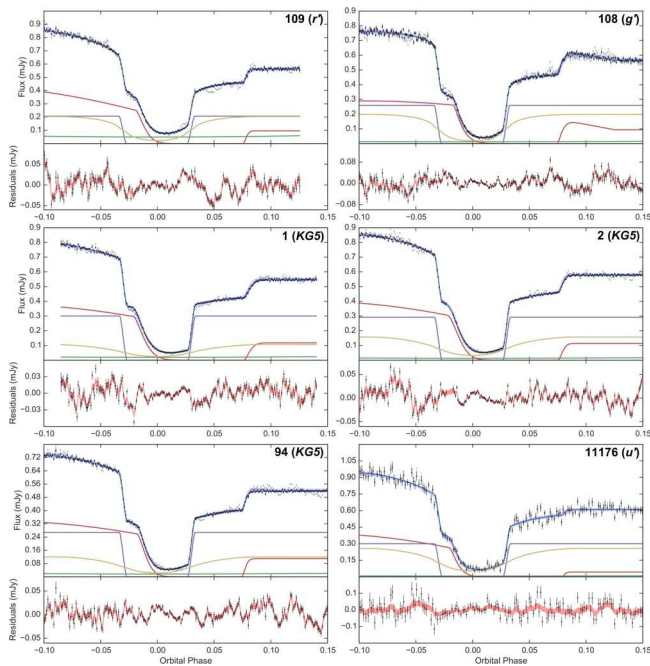
Figure A13. Simultaneous eclipse model fit to six SSS130413 eclipse light curves. See Section 4.1 for full details of what is plotted. Displayed in the top-right corner of each eclipse plot is the cycle number of the eclipse and the wavelength band it was observed in.
