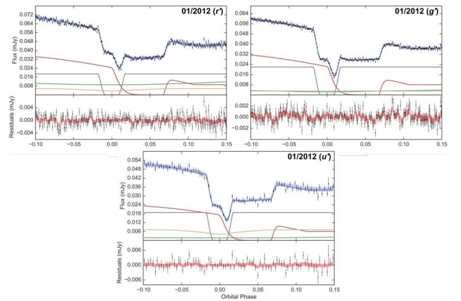
Figure A3. Simultaneous eclipse model fit to three average CSS110113 eclipse light curves. See Section 4.1 for full details of what is plotted. Displayed in the top-right corner of each average eclipse plot is the date and wavelength band each of the constituent eclipses were observed in.
