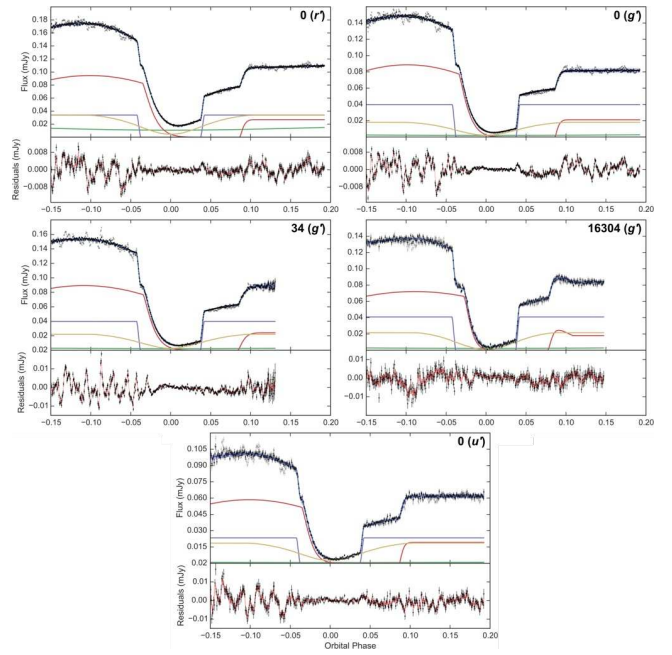
Figure A2. Simultaneous eclipse model fit to five CTCV 1300 eclipse light curves. See Section 4.1 for full details of what is plotted. Displayed in the top-right corner of each eclipse plot is the cycle number of the eclipse and the wavelength band it was observed in.
