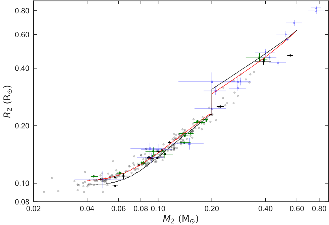
Figure 9. Measured CV donor masses ( M_2 ) and radii ( R_2 ). The data point colour/shape scheme is the same as in Figure 8. The red and black lines represent the best-fit ( f_{\text{GR}} = 2.47 \pm 0.22 , f_{\text{MB}} = 0.66 \pm 0.05 ) and ‘standard’ ( f_{\text{GR}} = f_{\text{MB}} = 1 ) evolutionary tracks from Knigge et al. (2011), respectively.
