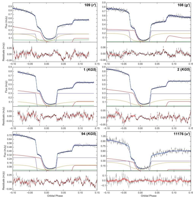
Figure A13. Simultaneous eclipse model fit to six SSS130413 eclipse light curves. See Section 4.1 for full details of what is plotted. Displayed in the top-right corner of each eclipse plot is the cycle number of the eclipse and the wavelength band it was observed in.
