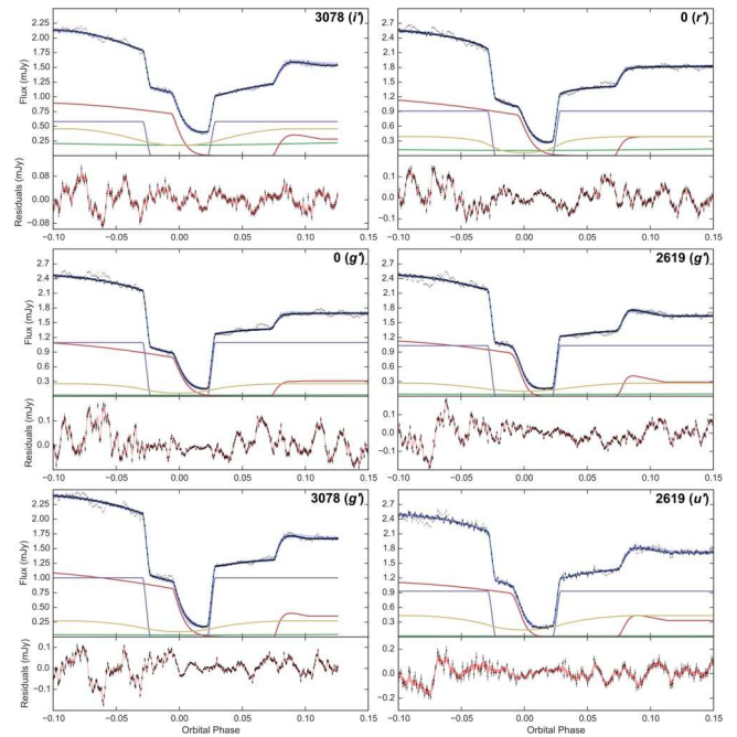
Figure A6. Simultaneous eclipse model fit to six OY Car eclipse light curves. See Section 4.1 for full details of what is plotted. Displayed in the top-right corner of each eclipse plot is the cycle number of the eclipse and the wavelength band it was observed in.
