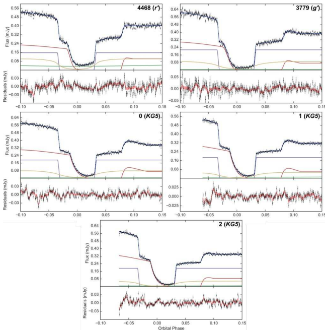
Figure A5. Simultaneous eclipse model fit to five IY UMa eclipse light curves. See Section 4.1 for full details of what is plotted. Displayed in the top-right corner of each eclipse plot is the cycle number of the eclipse and the wavelength band it was observed in.
