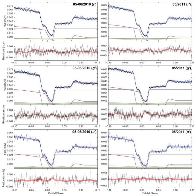
Figure A1. Simultaneous eclipse model fit to six average CSS080623 eclipse light curves. See Section 4.1 for full details of what is plotted. Displayed in the top-right corner of each average eclipse plot is the date(s) and wavelength band each of the constituent eclipses were observed in.
