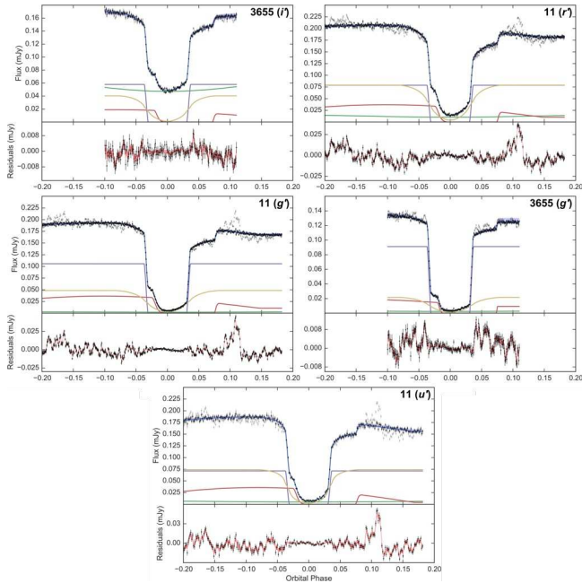
Figure A14. Simultaneous eclipse model fit to five V713 Cep eclipse light curves. See Section 4.1 for full details of what is plotted. Displayed in the top-right corner of each eclipse plot is the cycle number of the eclipse and the wavelength band it was observed in.
