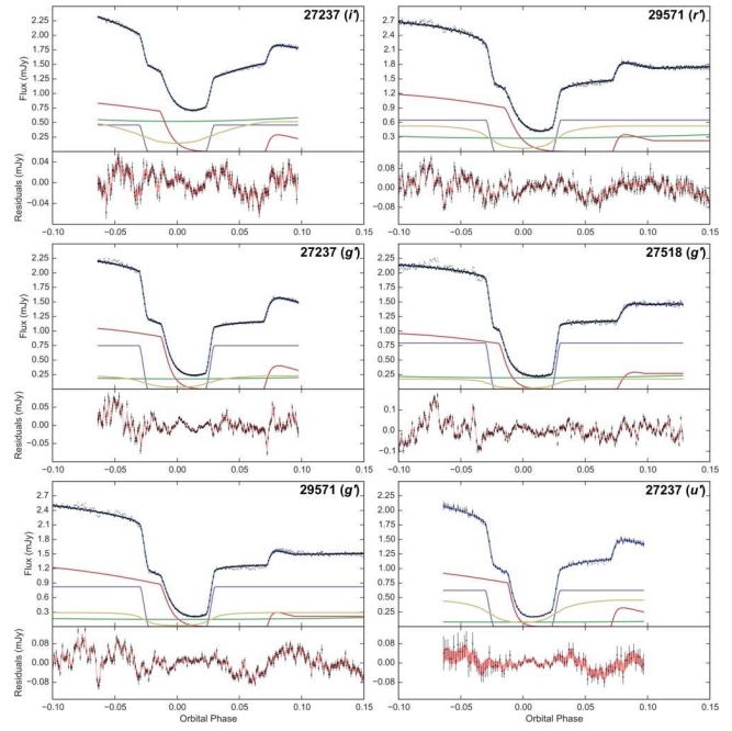
Figure A15. Simultaneous eclipse model fit to six Z Cha eclipse light curves. See Section 4.1 for full details of what is plotted. Displayed in the top-right corner of each eclipse plot is the cycle number of the eclipse and the wavelength band it was observed in.
