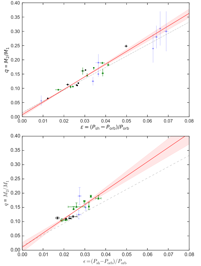
Figure 7. Measured \epsilon_{\text{B}} and q values of superhumping and eclipsing CVs, with the same data point colour/shape scheme as Figure 5. The dashed grey line shows the existing linear calibration of the \epsilon(q) relation for superhumping CVs from Knigge (2006), while the red line shows an updated calibration from this work. The red shaded region represents 1\sigma errors. The top plot shows the relationship for stage B superhumps, the bottom plot that for stage C superhumps.
