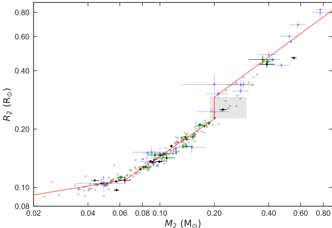
Figure 8. Measured CV donor masses ( M_2 ) and radii ( R_2 ). The data point colour/shape scheme is the same as in Figure 5, but with additional superhumping systems (grey points), for which error bars have been omitted for clarity. The red line is the semi-empirical mass-radius relation from this work. The grey shaded region contains systems assumed to lie within the period gap, and are therefore not included in the updated broken-power-law fit.
