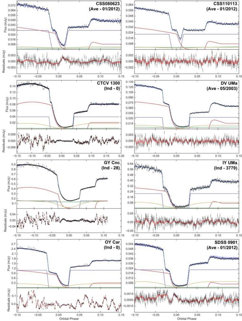
Figure 1. Eclipse model fits to g -band light curves of 15 CVs. The lightcurves are shown in grey points; see Section 4.1 for full details of what is plotted. The system name is displayed in the top-right corner of each plot, along with whether the eclipse is an individual (Ind) or average (Ave) eclipse. For individual eclipses the cycle number is shown, while for average eclipses the month and year of the eclipses is shown. See Appendix A for a complete set of eclipse plots.
