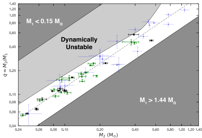
Figure 5. q vs M_2 plot for CVs. The grey regions are theoretically prohibited due to constraints put on M_1 . The dark grey regions cover unrealistically low white dwarf masses ( \lesssim 0.15 M_\odot ) and masses greater than the Chandrasekhar mass limit ( 1.44 M_\odot ), while the light grey region is forbidden by the empirical consequential angular momentum loss (eCAML) model of Schreiber et al. (2016). The dashed grey line represents the mean value of M_1 from this work. The green and black points represent masses obtained from eclipse modelling of ULTRACAM/ULTRASPEC data, either from this work (green) or otherwise (black). The faint blue points represent measured CV masses from other methods: eclipse modelling of other data (circles), contact phase timing (squares), and radial velocity (triangles).
