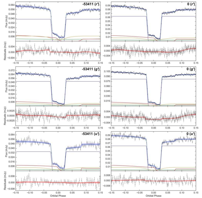
Figure A12. Simultaneous eclipse model fit to six SDSS 1501 eclipse light curves. See Section 4.1 for full details of what is plotted. Displayed in the top-right corner of each eclipse plot is the cycle number of the eclipse and the wavelength band it was observed in.
