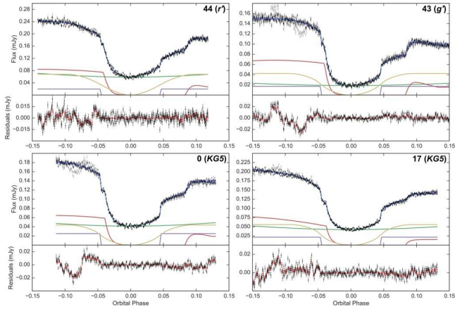
Figure A9. Simultaneous eclipse model fit to four SDSS 1006 eclipse light curves. See Section 4.1 for full details of what is plotted. Displayed in the top-right corner of each eclipse plot is the cycle number of the eclipse and the wavelength band it was observed in.
