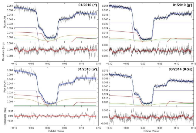
Figure A10. Simultaneous eclipse model fit to four average SDSS 1152 eclipse light curves. See Section 4.1 for full details of what is plotted. Displayed in the top-right corner of each average eclipse plot is the date and wavelength band each of the constituent eclipses were observed in.
