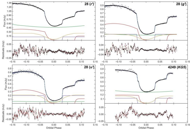
Figure A8. Simultaneous eclipse model fit to four GY Cnc eclipse light curves. See Section 4.1 for full details of what is plotted. Displayed in the top-right corner of each eclipse plot is the cycle number of the eclipse and the wavelength band it was observed in.
