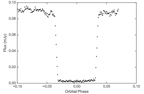
Figure 4. g' -band eclipse light curve (24 Jun 2015, cycle no. 11955) of V713 Cep during a low state.
