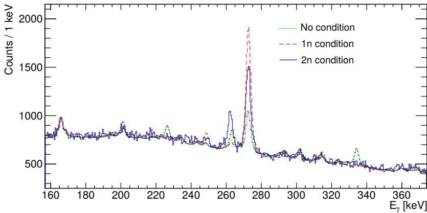
Fig. 3. (Colour on-line) Gamma spectra measured with AGATA spectrometer with a 115 MeV ^{36}\text{Ar} beam and ^{16}\text{O} target, without any condition (dotted green line) and gated on one and two neutrons (dashed red and solid blue lines, respectively) detected in the NEDA array. The spectra are scaled so the background level for all three of them is the same. The Y-axis scale is true for 1n gated spectrum. See discussion in the text.
