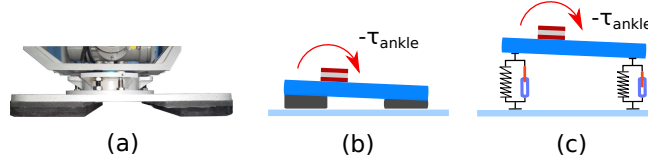
Fig. 7: Modeling of foot compliance: (a) real foot of the robot; (b) illustration of rubber deformation; (c) spring-damper models.
