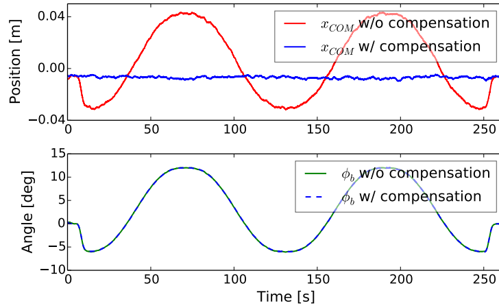
Fig. 15: Comparison of COM position without and then with the COM compensation during static torso attitude control.
