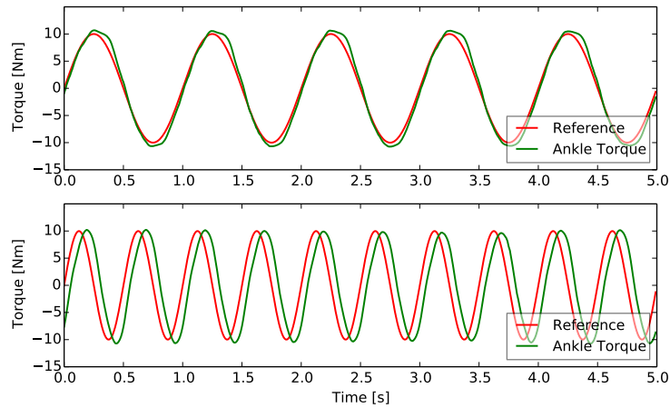
Fig. 13: Experiments of ankle torque tracking control.
