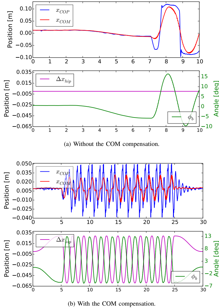
Fig. 17: Comparison of COM position without and then with the COM compensation during dynamic torso attitude control.
