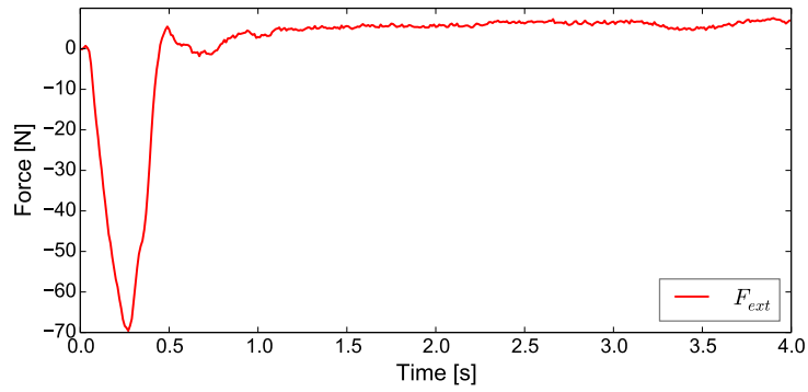
Fig. 21: External force measured in backward push recovery.
