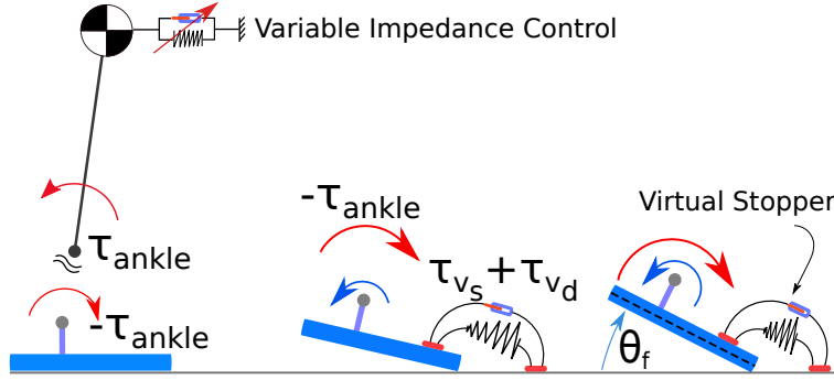
Fig. 9: Virtual mechanical stopper to prevent over-tilting.
