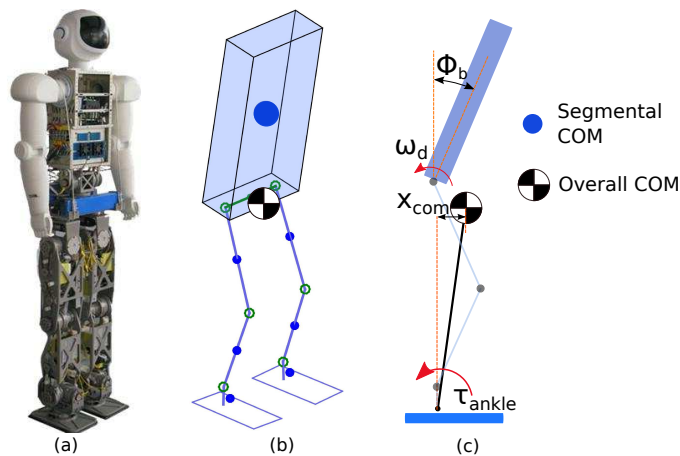
Fig. 2: KONG humanoid, the multi-mass model for COM state estimation, and the simplified model for the control design.
