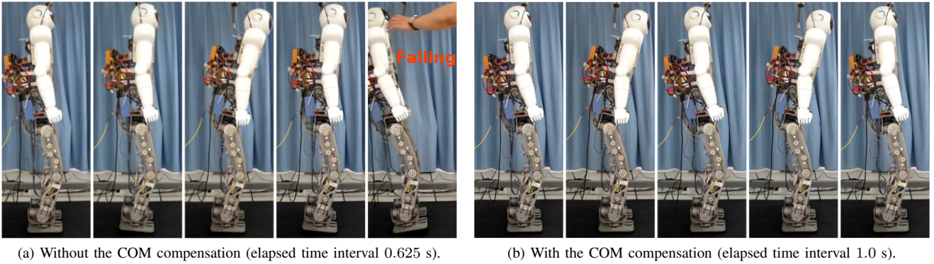
Fig. 16: Snapshots of different reactions without and then with the COM compensation.
