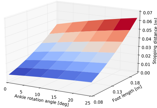
Fig. 5: Stopping distance, the horizontal distance between x_{\text{com}} when \dot{x}_{\text{com}} = 0 and the frontal edge of the foot, at a wide range of foot length and deliberately actuated ankle rotation.
