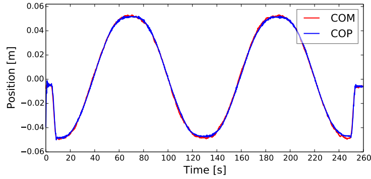
Fig. 11: Validation of COM estimation x_{\text{COM}} based on COP measurement x_{\text{COP}} during statically balanced motion in the sagittal plane.
