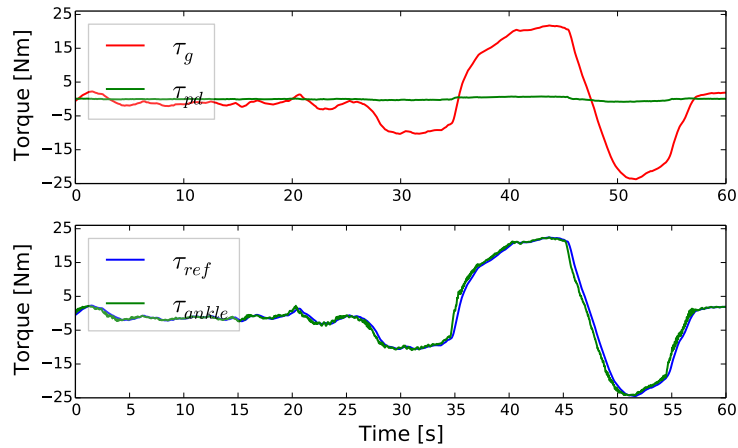
Fig. 14: Gravity compensation using COM estimation and ankle torque control.
