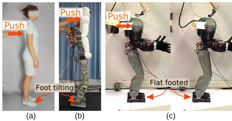
Fig. 1: The underactuation behaviors in human and humanoid push recoveries: (a) foot tilting observed from a person’s response; (b) a humanoid with our proposed control can perform human-comparable foot tilting; (c) the conventional balance control with flat-footed behavior.
