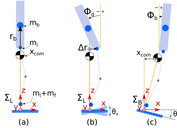
Fig. 10: Analytic COM compensation for torso motion using a three-mass model: (a) definition of local coordinate \Sigma_L used in inverse kinematics; (b) \Delta r compensation from (19) in the local coordinate \Sigma_L ; (c) observation from the state estimation integrated with IMU data in base coordinate \Sigma_B whose orientation aligns with the world coordinate.
