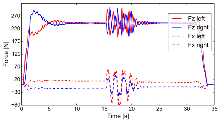
Fig. 18: Validation of vertical leg force control.
