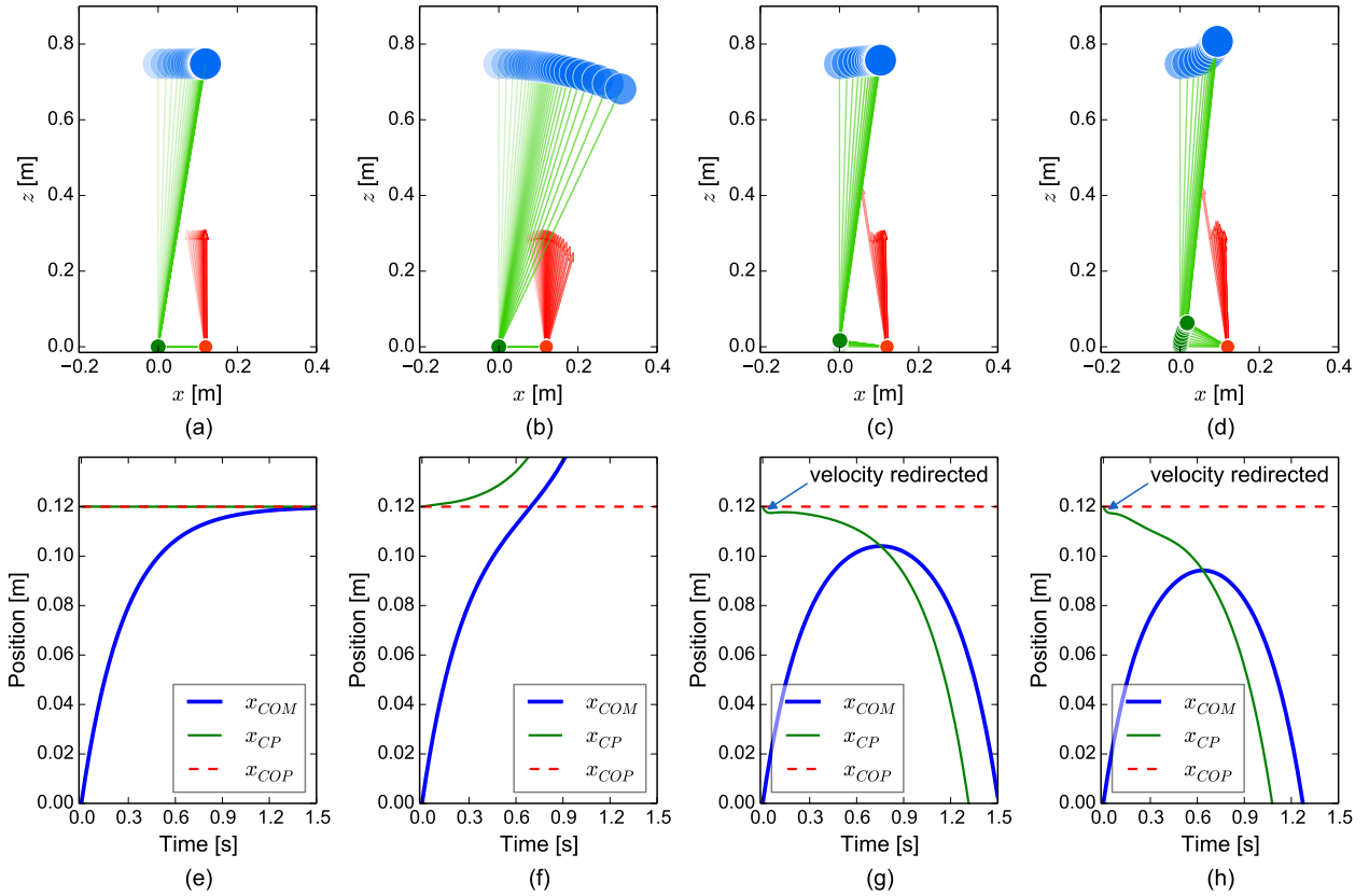
Fig. 4: Time-lapse illustration of the foot tilting effects: (a) flat foot with constant COM height; (b) flat foot with constant leg length; (c) foot tilting around toe with fixed ankle joint (zero COM velocity at 0.104 m); (d) active foot tilting around the edge of the foot with rotation of ankle joint (zero COM velocity at 0.093 m).
