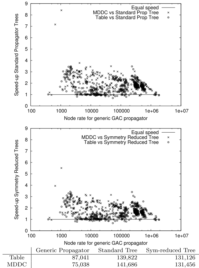
Fig. 7. XCSP experiment comparing MDDC and Table to both standard and symmetry-reduced propagator trees for all benchmarks with more than 100 nodes of search. The x -axis represents the node rate without propagator trees for the generic GAC propagator. The y -axis is the speed-up factor obtained when propagator trees are used. The table gives the geometric mean of the node rate for each configuration.
