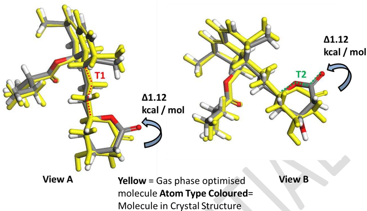
Figure 2 Conformational overlay of the gas phase optimised lovastatin molecule (yellow) and the molecule in the asymmetric unit of lovastatin (coloured by atom type) highlighting the conformational change of the tetrahydropyran ring through torsion 2 (T2 Green)
