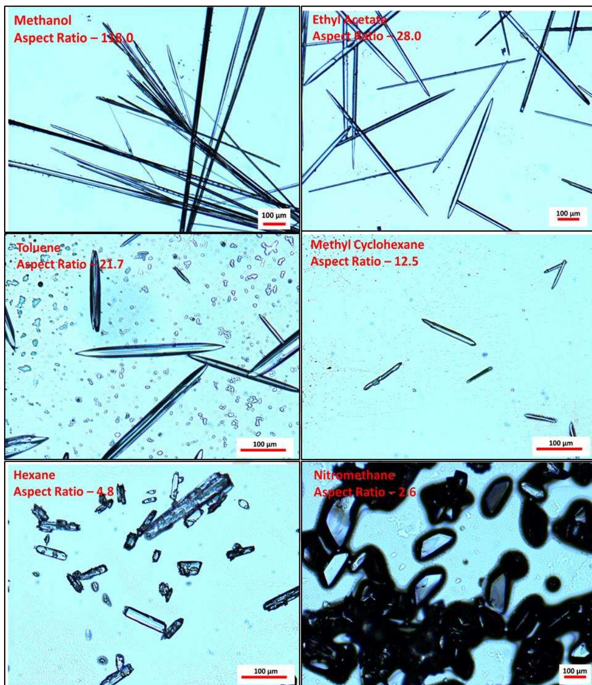
Figure 6 Micrographs of lovastatin crystals grown by slow solvent evaporation from, methanol (aspect ratio 118.0), ethyl acetate (aspect ratio 28.0), toluene (aspect ratio 21.7), methyl cyclohexane (aspect ratio 12.5), hexane (aspect ratio 4.8) and nitromethane solutions (aspect ratio 2.6), the approximate aspect ratio of the crystals were calculated by the ratio of the approximate length and width of the crystals
