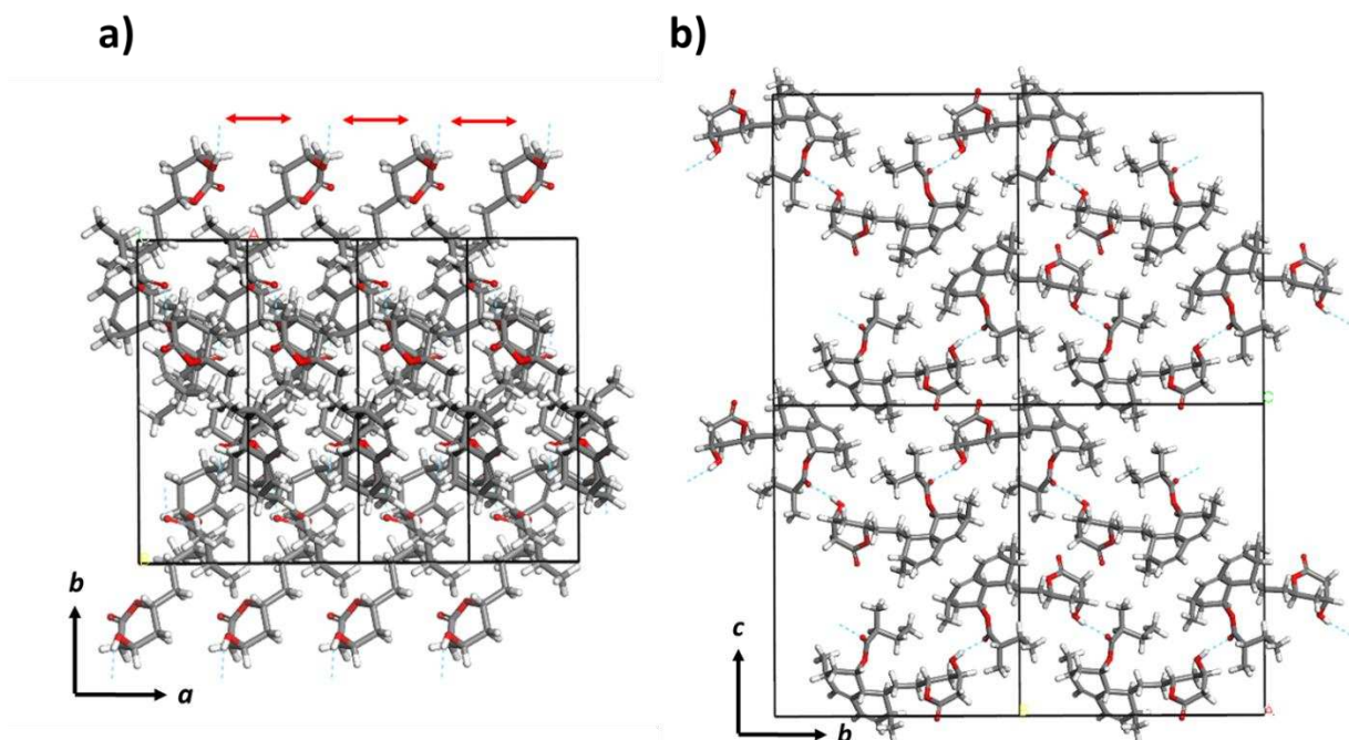
Figure 1 a) the crystal structure of lovastatin viewed down the crystallographic c axis highlighting the close stacking of the hexahydronaphthalene rings (red arrows) along the a axis and b) view down the crystallographic a axis highlighting the hydrogen bond between the S-butanoate ester group and the alcohol functionality
