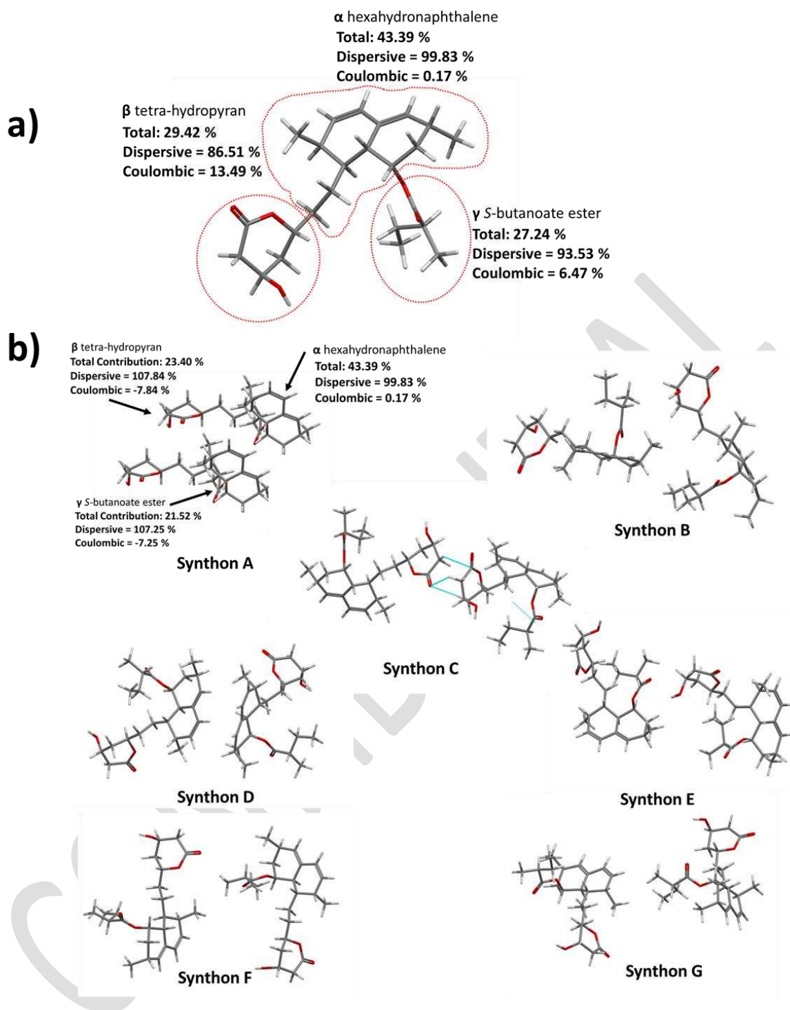
Figure 4 a) The percentage contribution to the lattice energy provided by the 3 functional groups of the lovastatin asymmetric unit, and the breakdown of each to dispersive and coulombic contribution to the total, b) The top seven intermolecular synthons which contribute to the lattice energy of lovastatin, ranked as a function of total interaction energy, Synthon A shows the breakdown of the total contribution of the three main functionality's (as identified in a)) of the lovastatin molecule towards the overall intermolecular interaction energy together with the percentage contribution of the dispersive and coulombic components of those functionality's
