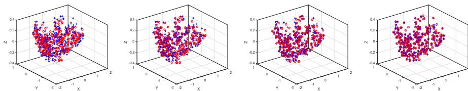
Figure 9. Registration results obtained from the application of pair-wise rivals on a specific example generated from 3D COPD data. Initial unregistered point sets (first column) and the results of CPD (second column), CPD-GL (third column), and SCGF (fourth column).
