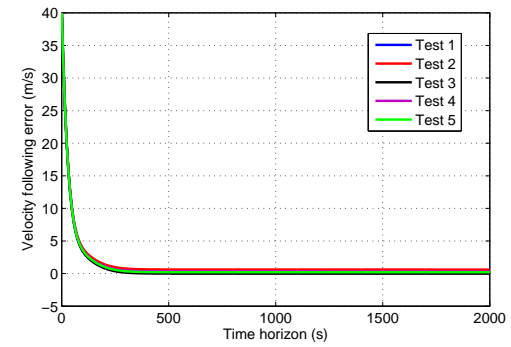
(d) Velocity tracking error between train 2 and train 3
