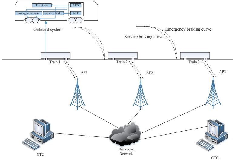
Figure 1: Illustration of train control systems with train-to-ground communication
