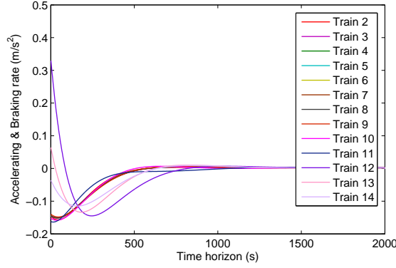
Figure 9: Curves of accelerating and braking rates
