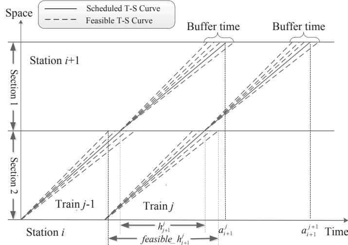
Figure 2: Train following scenario
