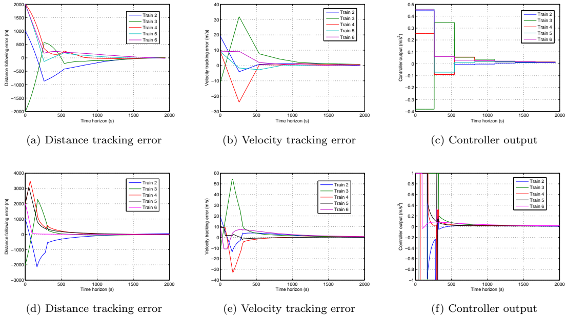
Figure 11: Comparison between the performance of SMPC (a-c) and LQ (d-f) for Instance 2.
