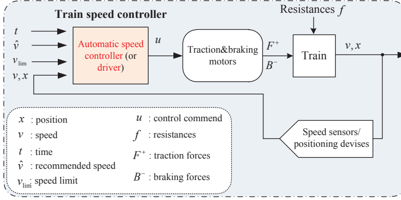
Figure 4: Illustration of railway train control model
