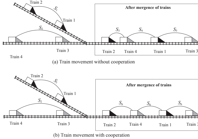
Figure 3: Headway adjustment for multiple train control problem. The boxed area after the merge shows the train sequence and headway.
