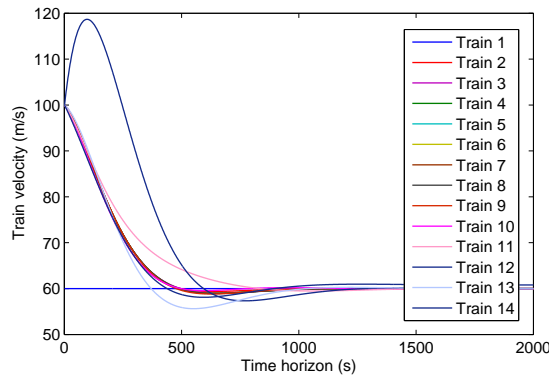
Figure 8: Time-velocity curves with train cooperative control
