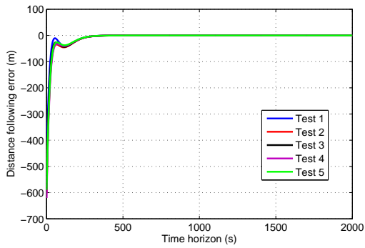
(c) Distance tracking error between train 2 and train 3
