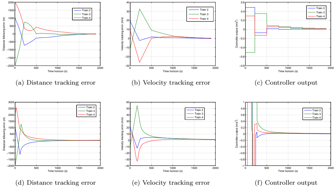
Figure 10: Comparison between the performance of SMPC (a-c) and LQ (d-f) for Instance 1.
