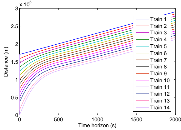
Figure 7: Illustration of time-space diagram of multiple trains
