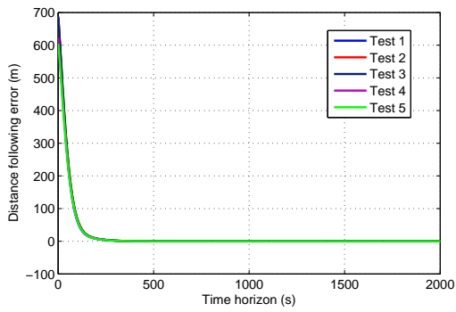
(a) Distance tracking error between train 1 and train 2
