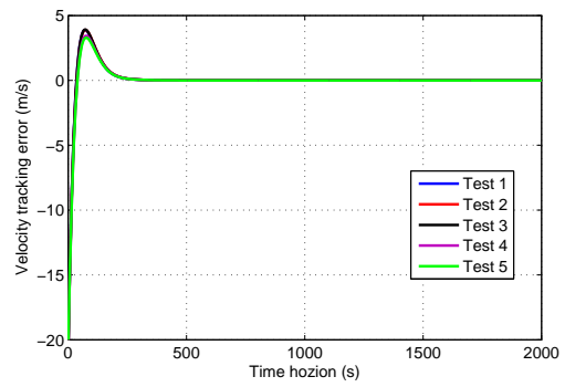
(b) Velocity tracking error between train 1 and train 2
