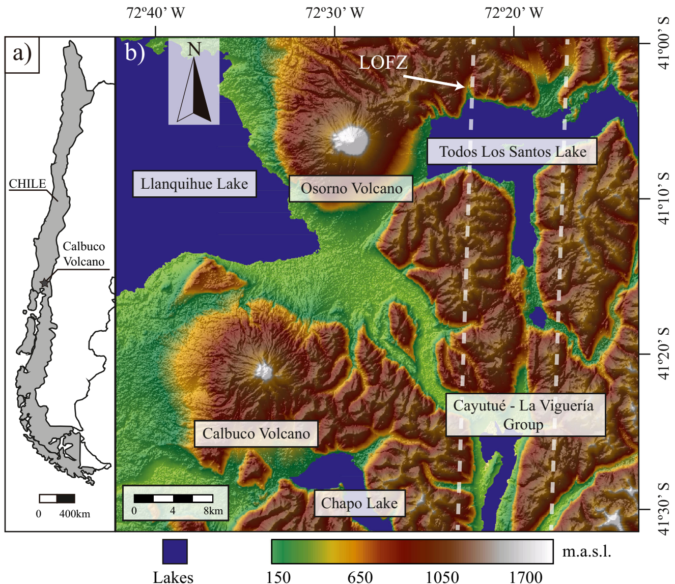
Fig. 1 (a) Location of Calbuco volcano with respect to Chile and (b) regional map of Calbuco volcano on shaded relief/Digital Elevation Model. Calbuco is located between Llanquihue and Chapo lakes, ~20 km west from the Llanquihue–Ofqui Fault Zone (LOFZ, dashed white
