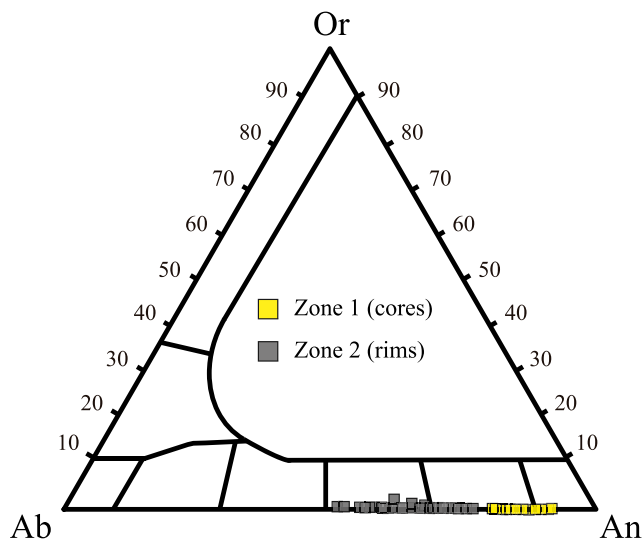
Figure 4 Plagioclase compositions of the studied samples. Zone 1 represents core compositions of group I, whereas zone 2 represents rim compositions of group I and the whole-crystal composition of group II
