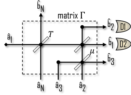
Fig. 4. The quantum channel and the QS are considered as a combined system with input modes \hat{a}_1 - \hat{a}_3 and \hat{a}_N and output modes \hat{b}_1 - \hat{b}_3 and \hat{b}_N . The transformation matrix of the system is given by (4).
