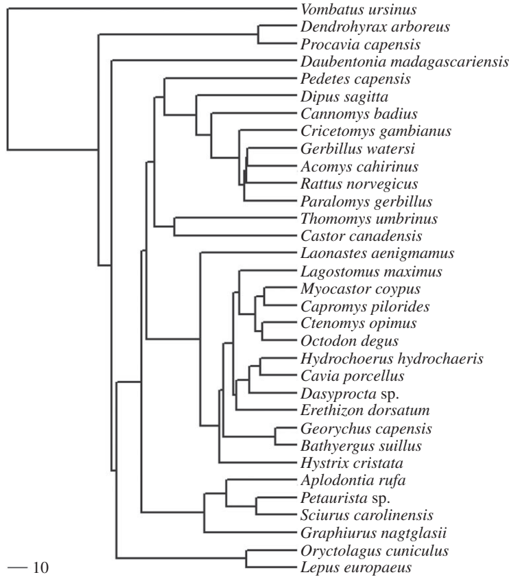
Figure 2. Phylogeny of species used in this analysis. Scale bar represents 10 million years.
