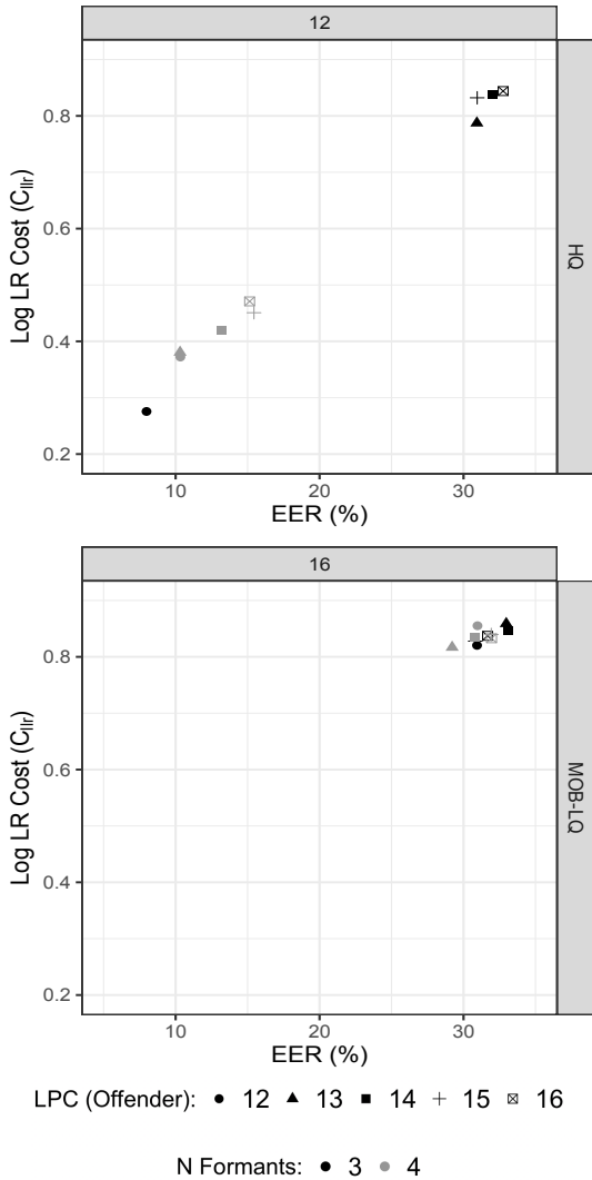
Figure 1: System validity (EER and C_{llr} ) in the most (top: HQ-HQ, Suspect LPC = 12) and least (bottom: HQ-MOB LQ , Suspect LPC = 16) variable conditions
