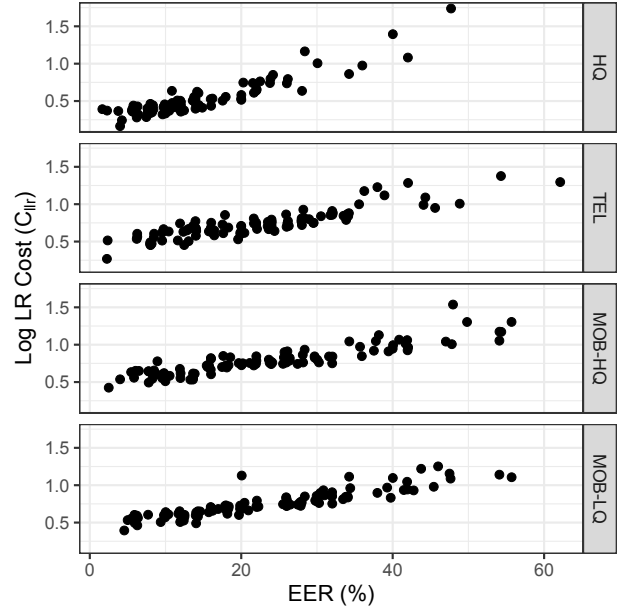
Figure 2: Speaker-specific system validity (EER and C_{llr} ) in the four transmission conditions (each dot represents a single speaker and is calculated using their SS and DS LLRs across all settings)
