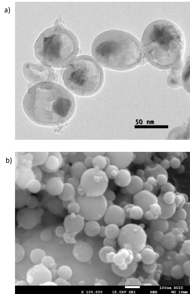
Figure 1. a) TEM and b) SEM micrographs of Al-Cu nePCM
