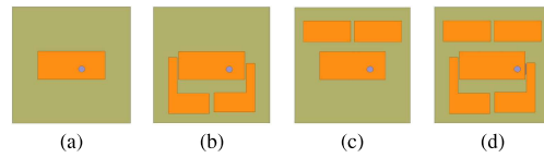
Fig. 2: The procedure of adding the parasitic elements to improve the antenna bandwidth performance in which case 1 is shown in (a), case 2 in (b), case 3 in (c), case 4 in (d).
