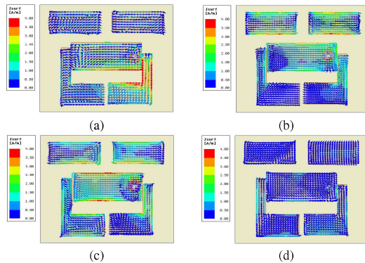
Fig. 4: Simulated surface current of the proposed antenna at (a) 4.7GHz, (b) 6.5 GHz, (c) 7.5 GHz, and (d) 8.615 GHz .
