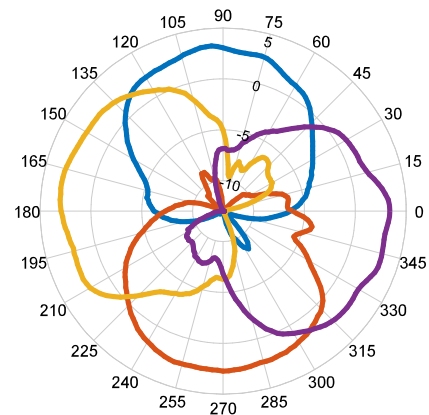
Fig. 23: Measured radiation pattern of the switchable directional antenna system at 5 GHz (co-polarisation xz plane) [17].
