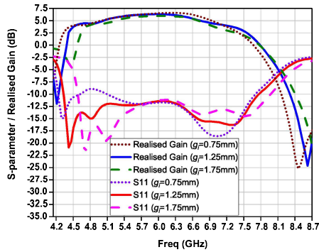
Fig. 11: Simulated reflection coefficients and realised gain for different gap separation of L-shaped parasitic elements and driven patch ( g_p ).
