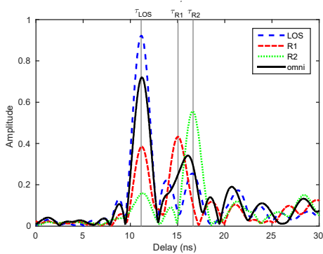
Fig. 24: Measured impulse response steering the antenna's mainlobe in the direction of the LOS (blue, dashed), reflection R1 (red, dotted dashed) and reflection R2 (green, dotted). The impulse response measured with an omnidirectional antenna (black, solid) is shown for comparison.
