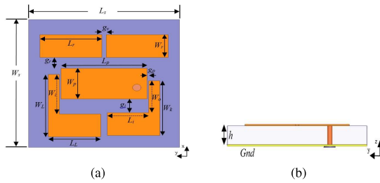
Fig. 1: Configuration of the proposed broadband microstrip filtering antenna with L- and rectangular-shaped parasitic elements. (a) Top view. (b) side view.
