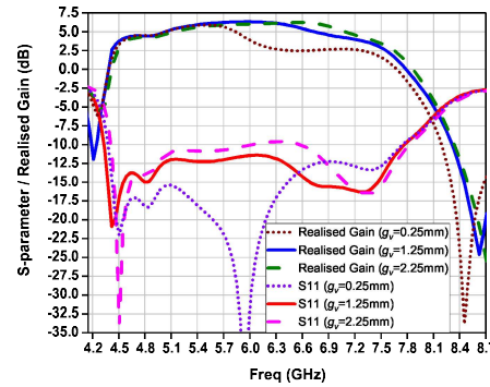
Fig. 13: Simulated reflection coefficients and realised gain for different gap separation between rectangular parasitic elements ( g_v ).
