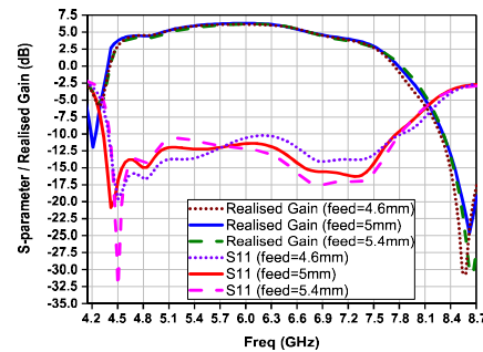
Fig. 10: Simulated reflection coefficients and realised gain for different positions of feeding probe.
