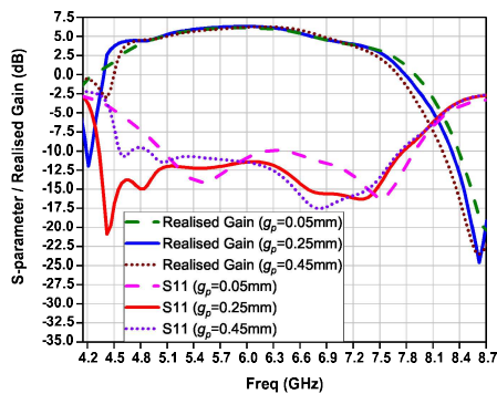
Fig. 12: Simulated reflection coefficients and realised gain for different gap separation of L-shaped parasitic elements and driven patch ( g_p ).
