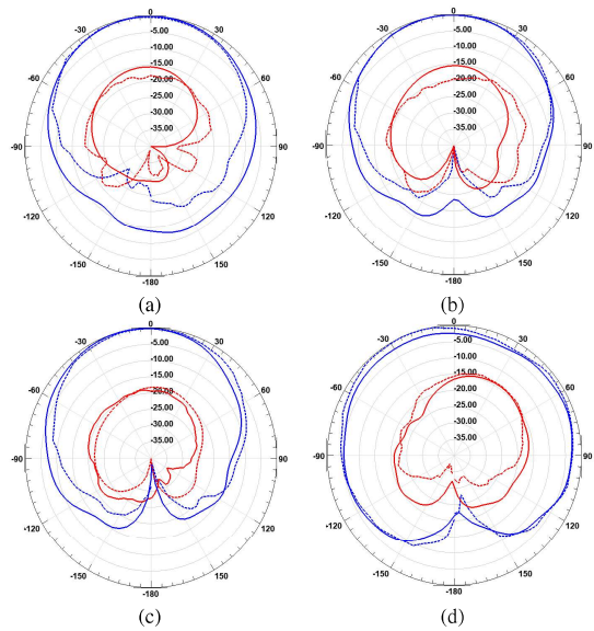
Fig. 19: Simulated and measured radiation patterns where solid and dashed blue lines represent simulated and measured co-polarisation (xz-plane) respectively: (a) 4.7 GHz, (b) 5.5 GHz, (c) 6 GHz, and (d) 7.5 GHz.
