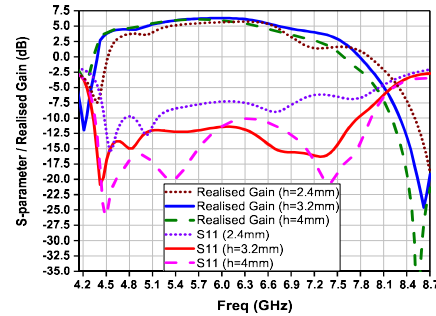
Fig. 9: Simulated reflection coefficients and realised gain for different sizes of substrate height.
