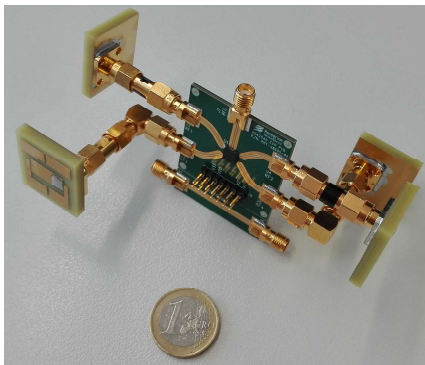
Fig. 22: Directional antenna system containing four antennas and the RF switching network [17].
