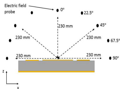
Fig. 20: Side view of the proposed antenna showing electric field probes.
