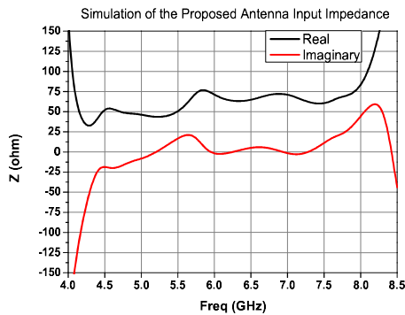
Fig. 7: Simulated response of real and imaginary part of the antenna input impedance.
