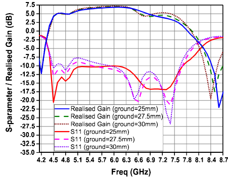
Fig. 15: Simulated reflection coefficients and realised gain as a function of ground size.
