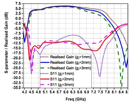
Fig. 14: Simulated reflection coefficients and realised gain for different gap separation of rectangular parasitic elements to driven patch ( g_r ).
