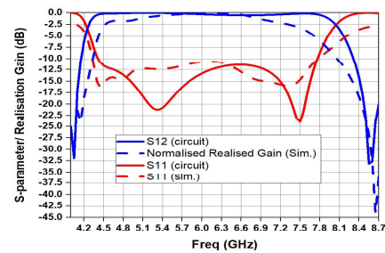
Fig. 6: Simulation and theoretical reflection/transmission coefficients and normalised realised gain of the proposed antenna
