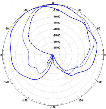
Fig. 16: Simulated radiation pattern at 7.2 GHz for different increase of ground size as follows: solid line (0mm), dotted line (5mm), and dashed line (10mm).
