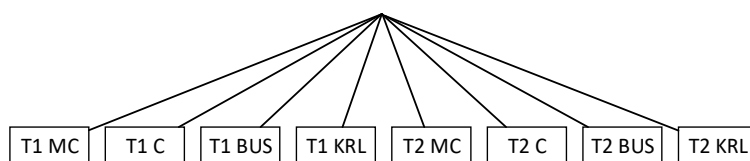
Figure 1. Multinomial logit model structure.
