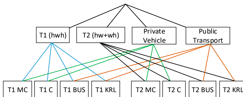
Figure 3. Cross-nested logit model structure.
